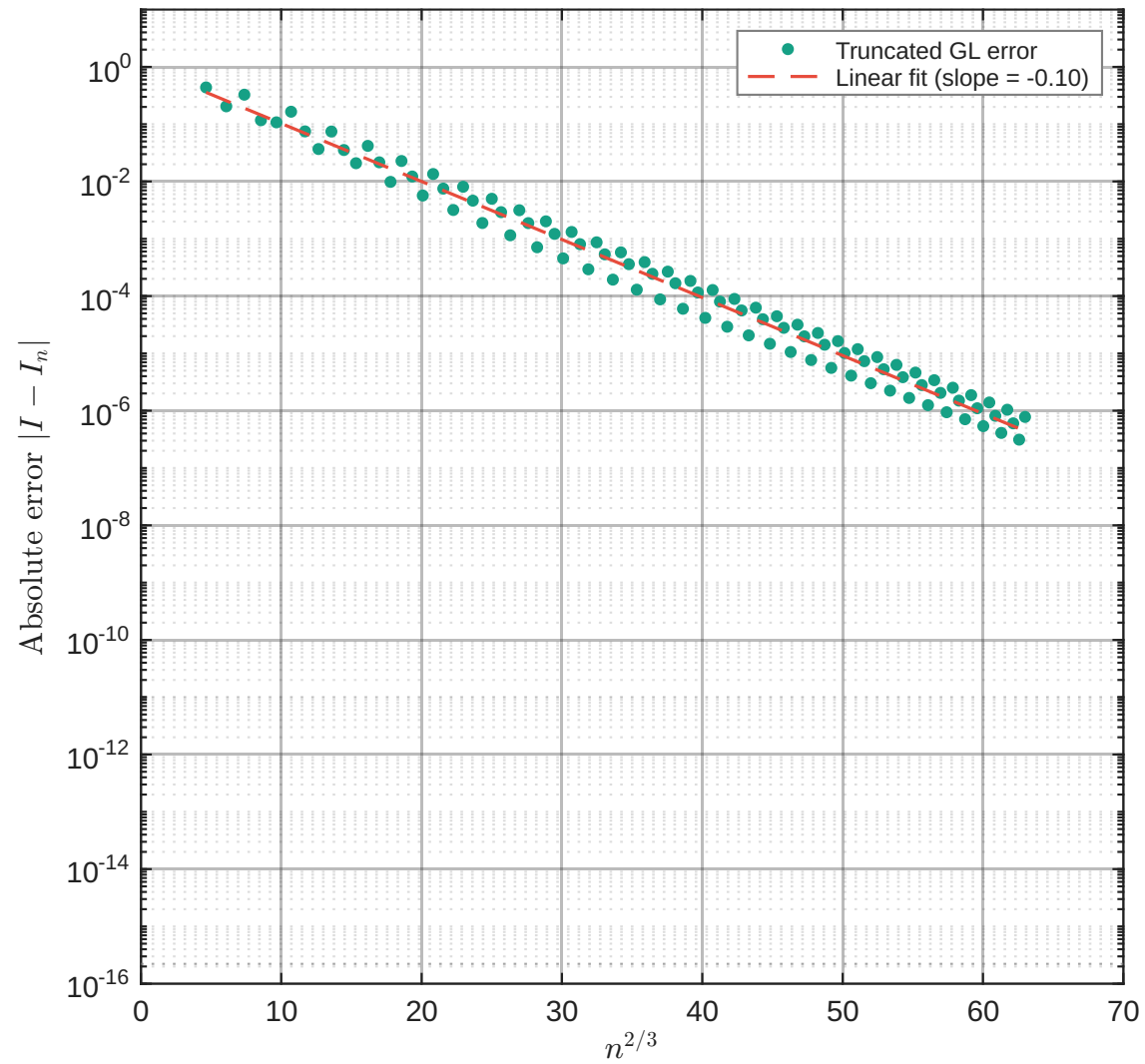
(b) Truncated GL: O(e^{-Cn^{2/3}})
