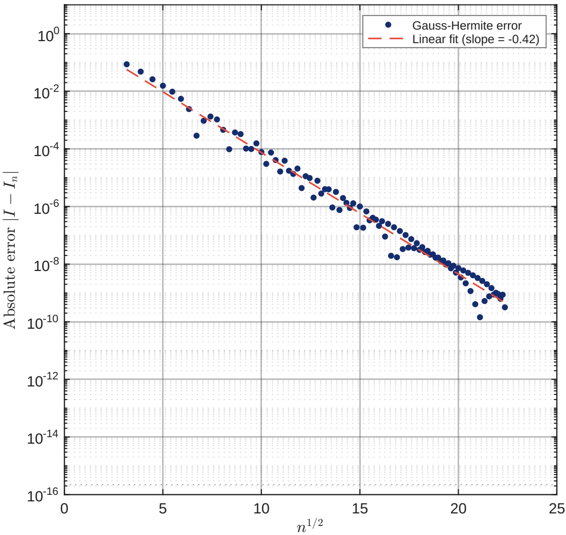
(a) Gauss-Hermite: O(e^{-C\sqrt{n}})
