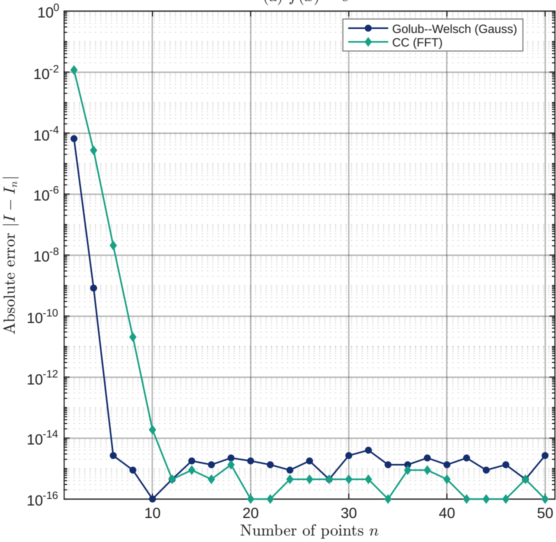
(a) f(x) = e^x
