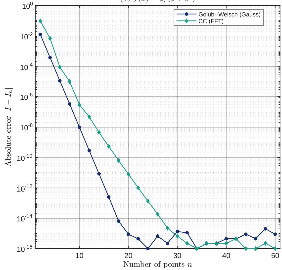
(b) f(x) = 1/(1+x^2)
