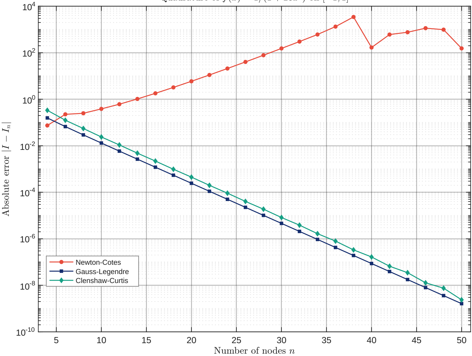
Quadrature of f(x) = 1/(1 + 25x^2) on [-1, 1]
