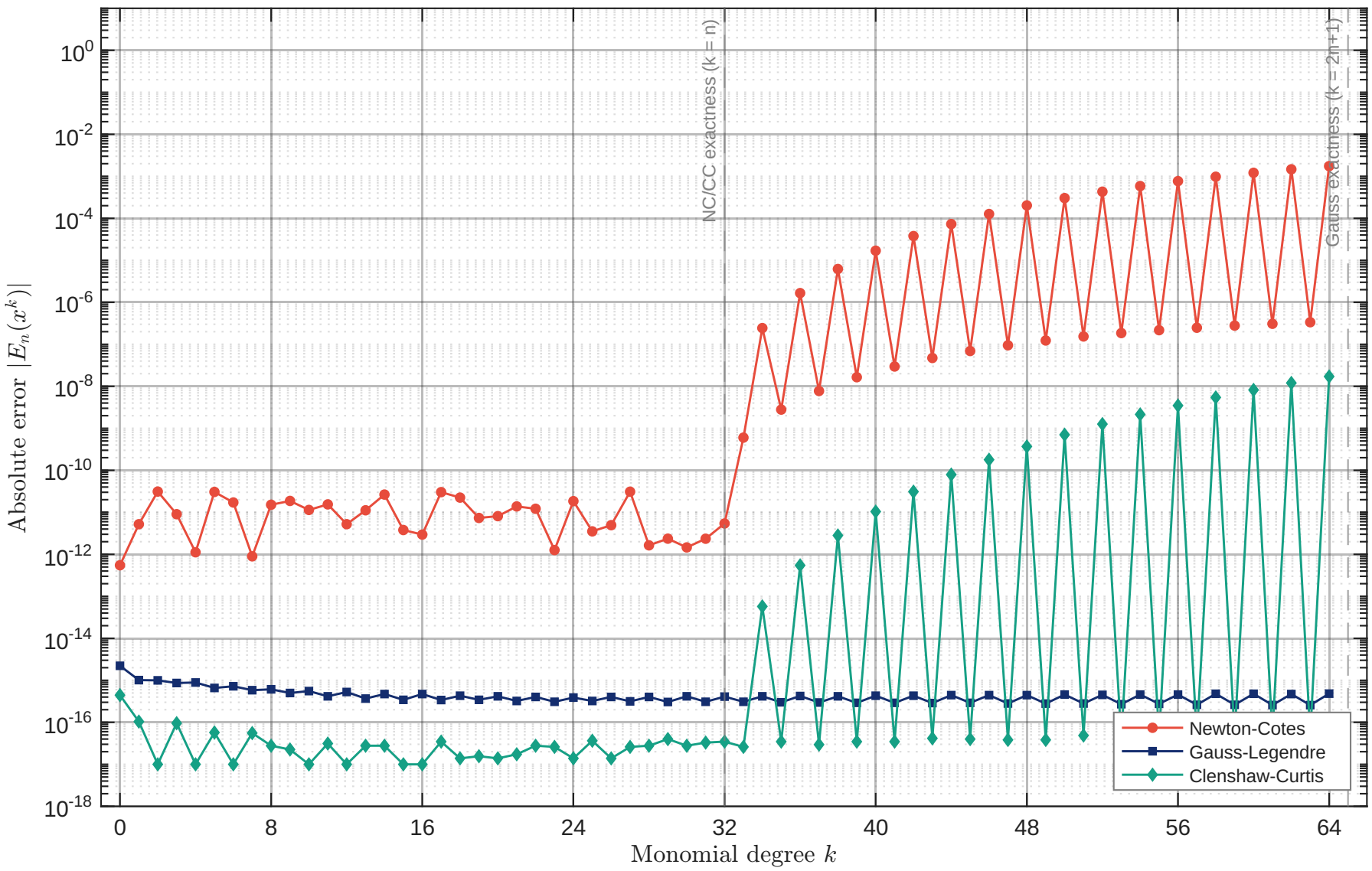
Polynomial exactness of three quadrature rules ( n + 1 = 33 points)
