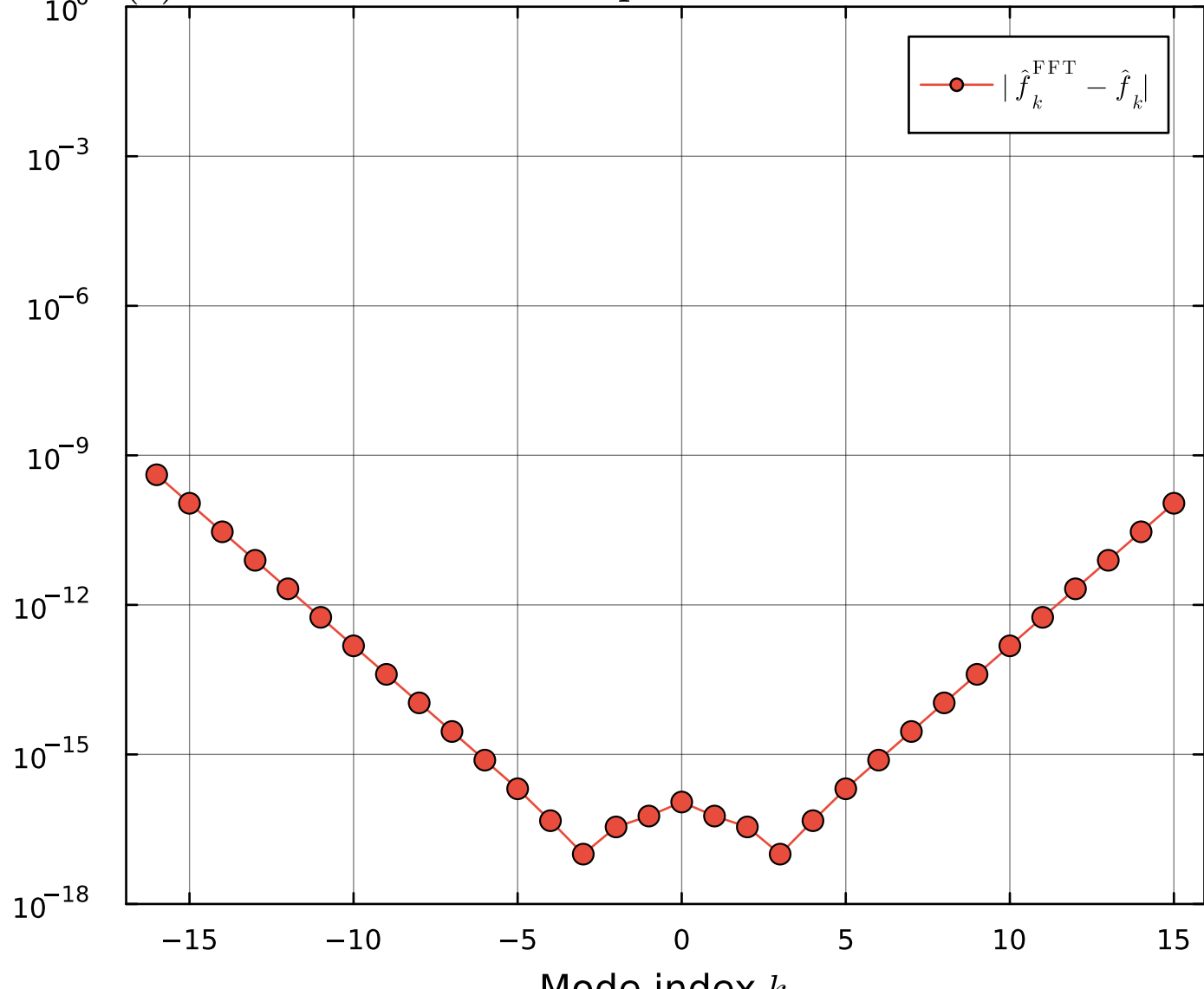
(b) FFError : machine precision in the resolved band
