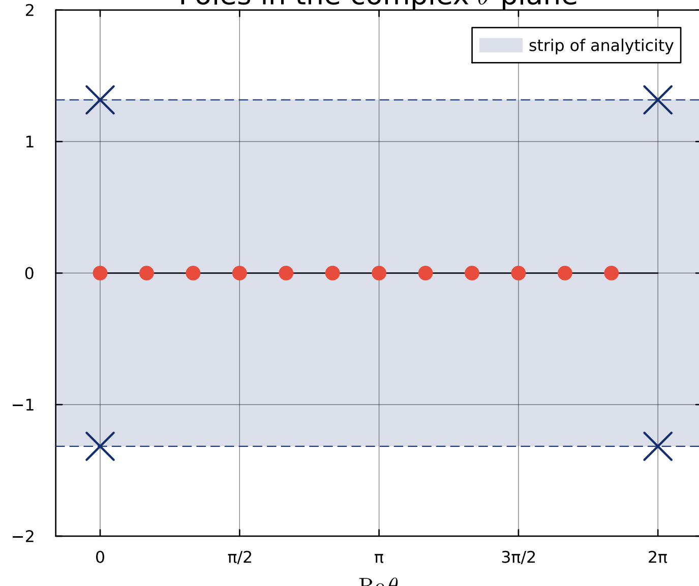
Poles in the complex \theta -plane
