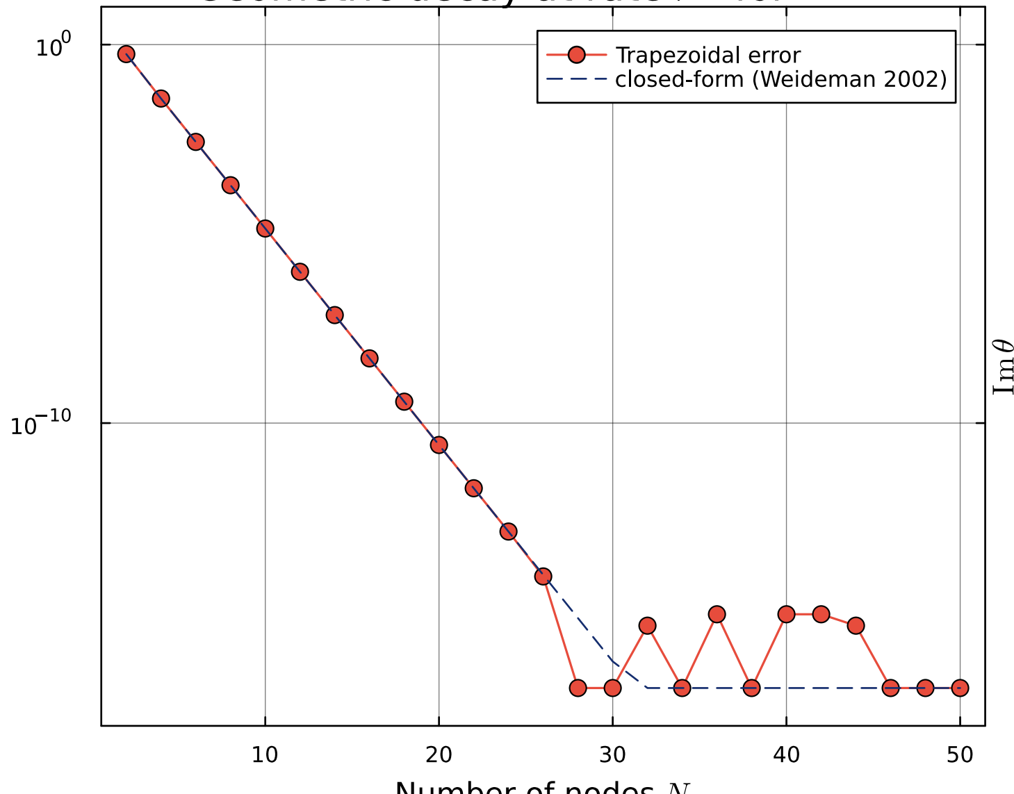
Geometric decay at rate r^N for a = 2
