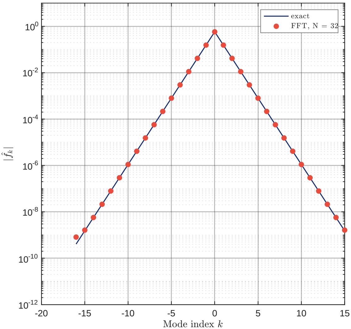
(a) Fourier-coefficient magnitudes for 1/(2 - \cos x)
