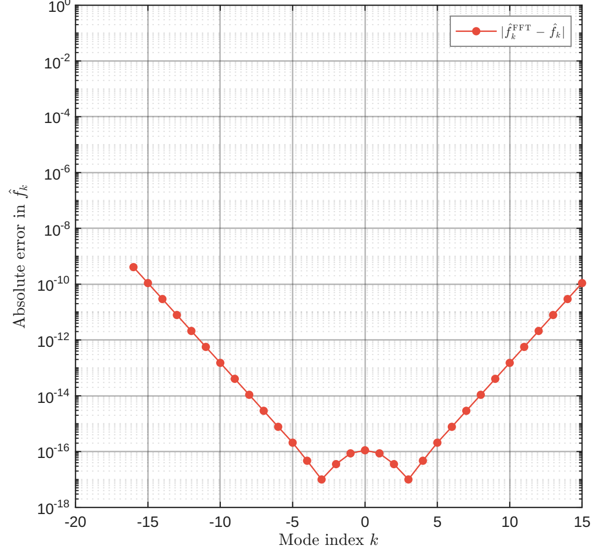
(b) FFT error: machine precision in the resolved band
