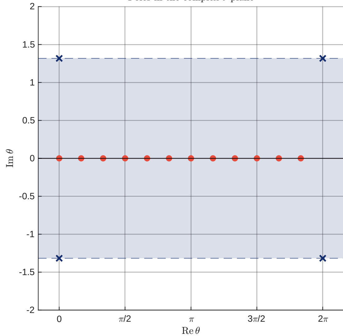
Poles in the complex \theta -plane
