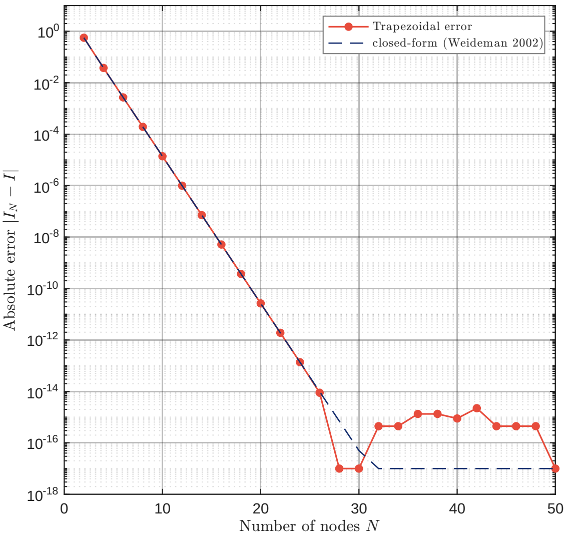
Geometric decay at rate r^N for a = 2
