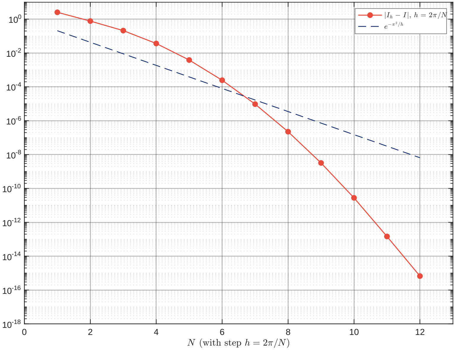
Real-line trapezoidal rule on e^{-x^2}/\sqrt{\pi}
