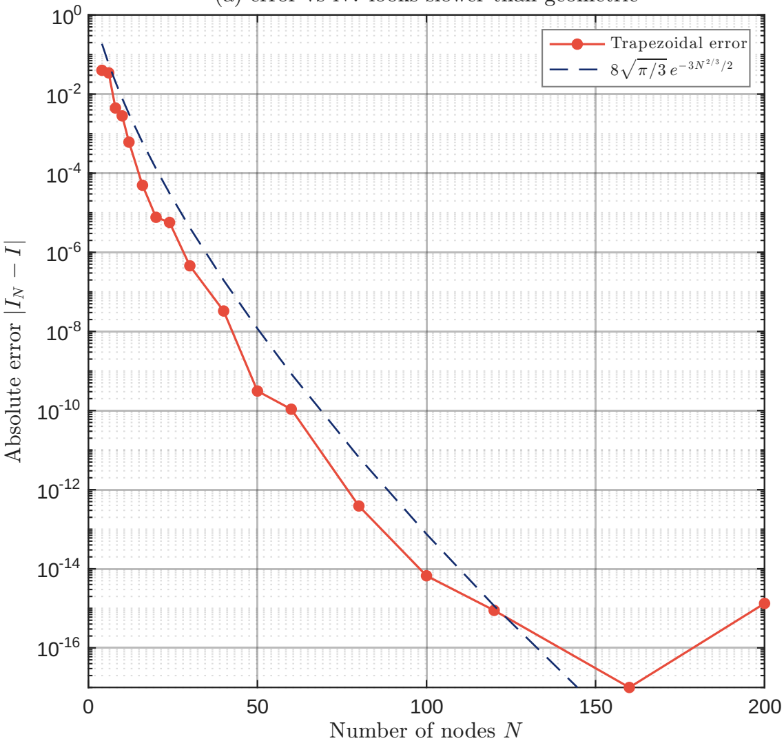
(a) error vs N : looks slower than geometric
