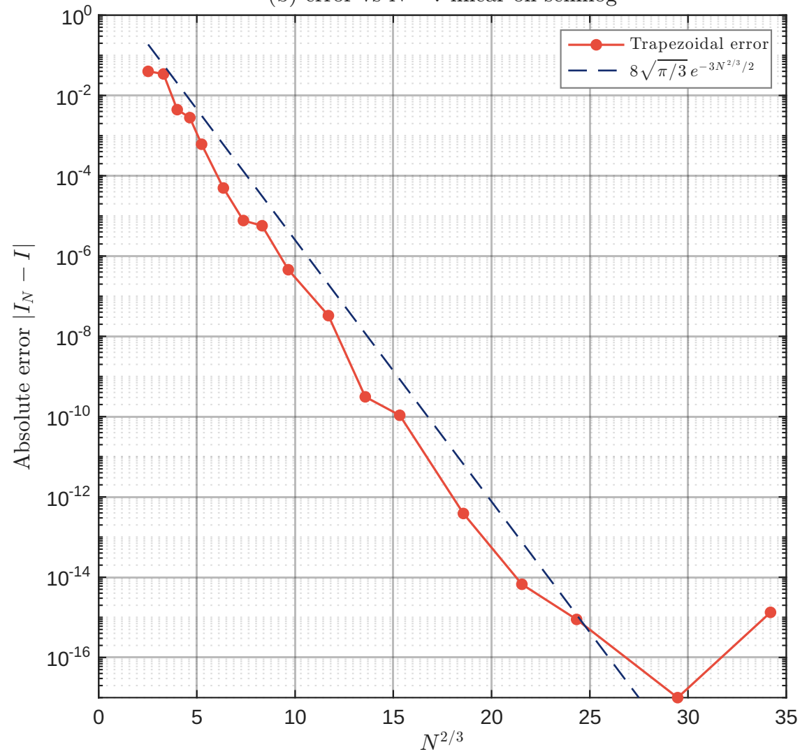
(b) error vs N^{2/3} : linear on semilog
