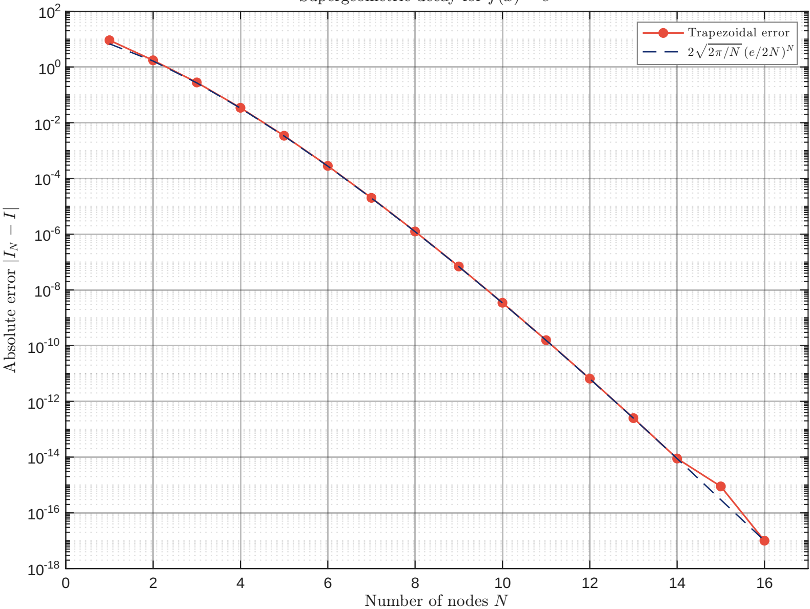
Supergeometric decay for f(x) = e^{\cos x}
