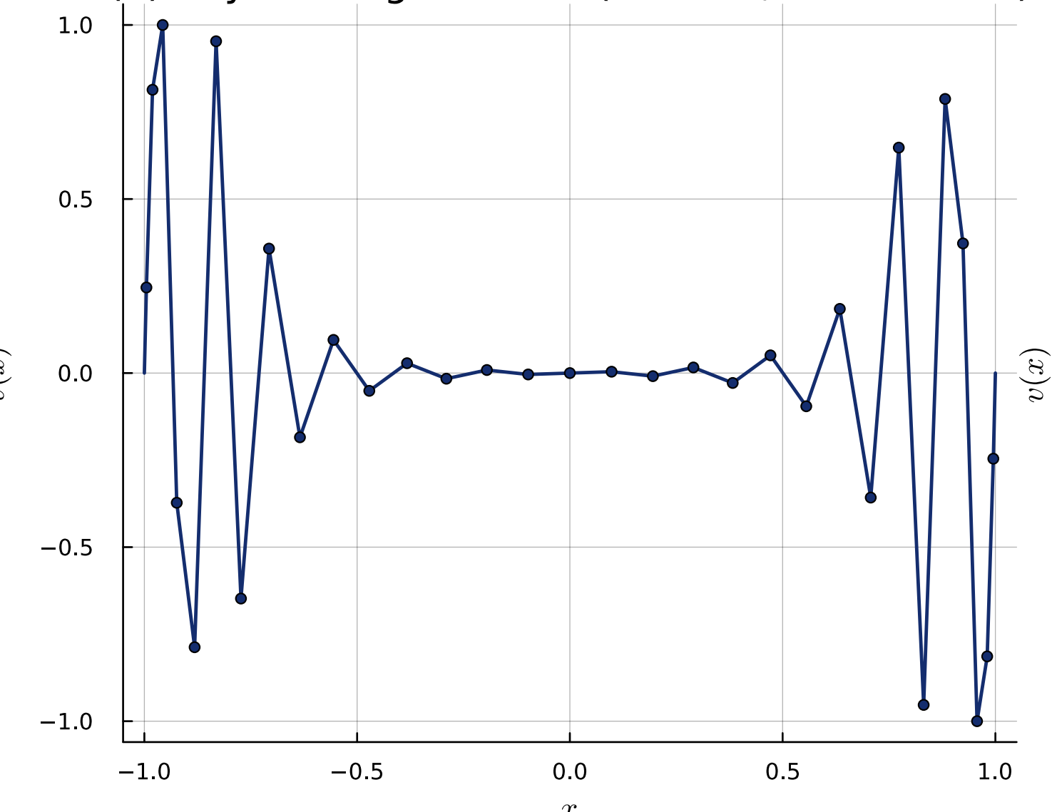
(a) Physical eigenvector (mode 8, \lambda = -2073.2 )
