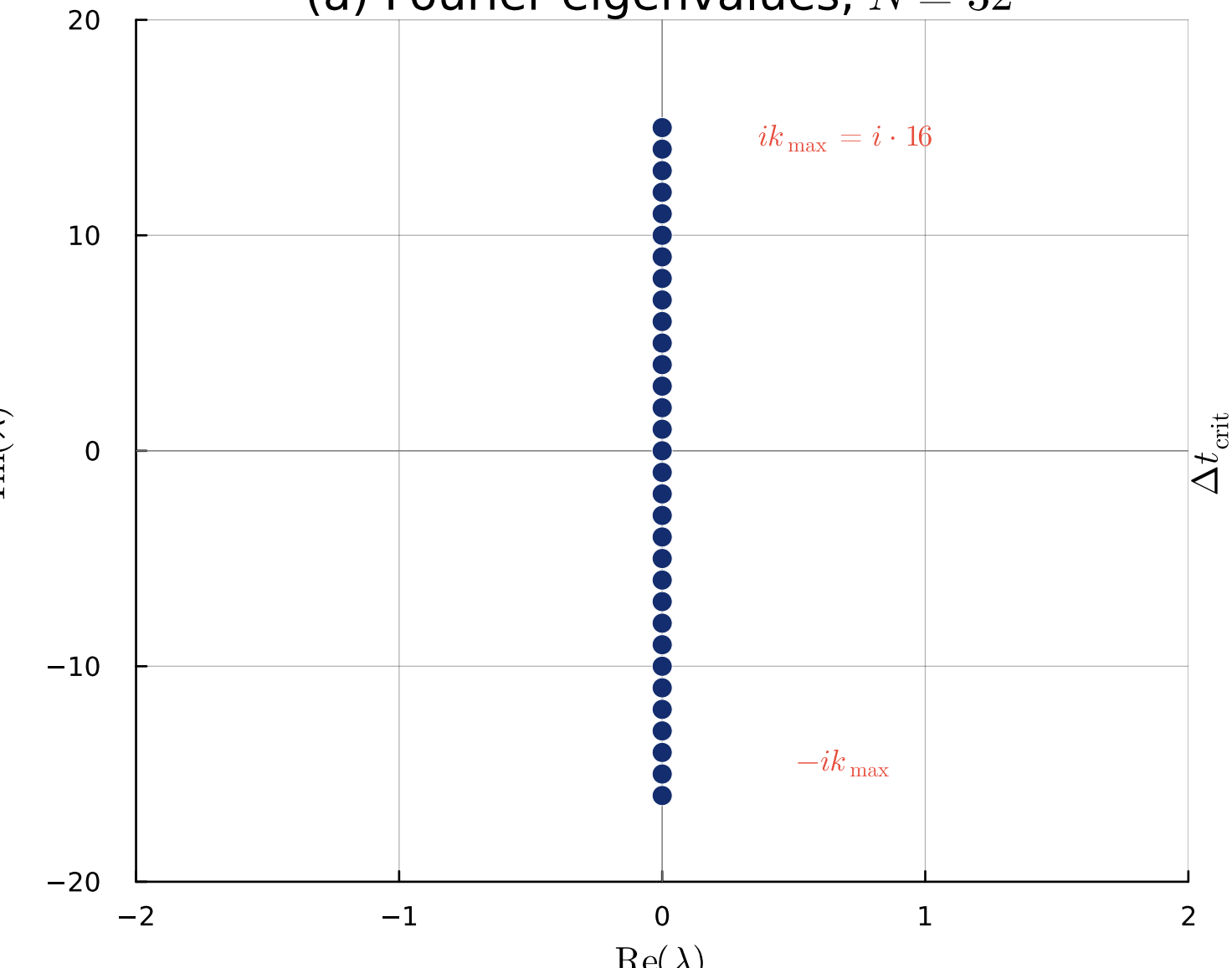
(a) Fourier eigenvalues, N = 32
