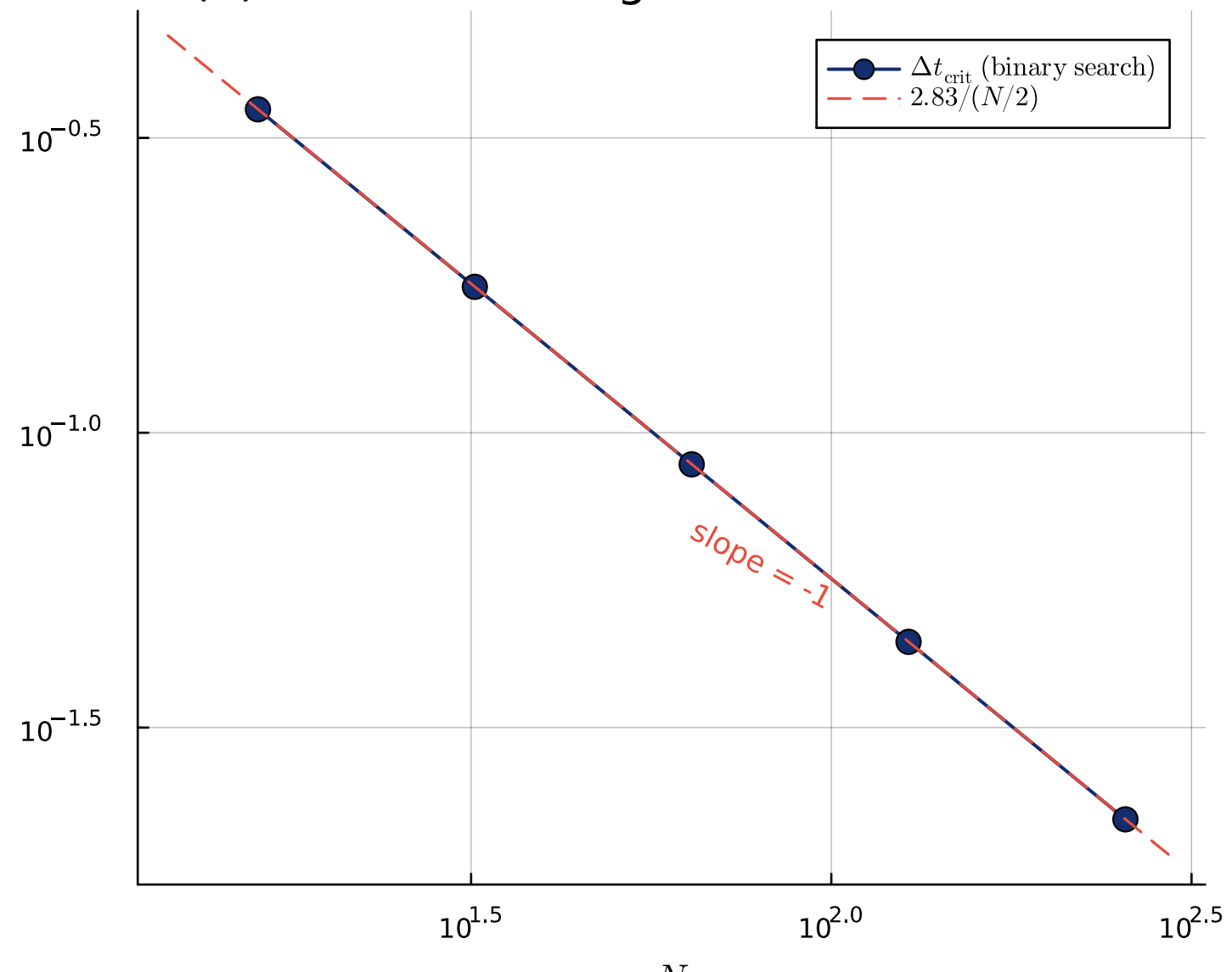
(b) RK4 CFL scaling for Fourier advection
