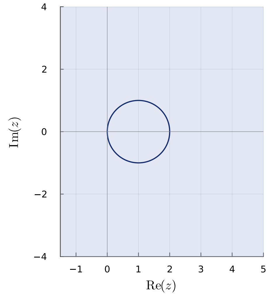
(f) Backward Euler
