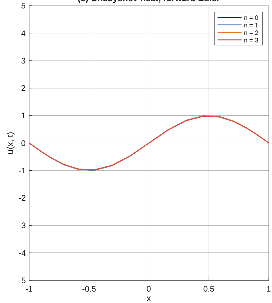
(c) Chebyshev heat, forward Euler
