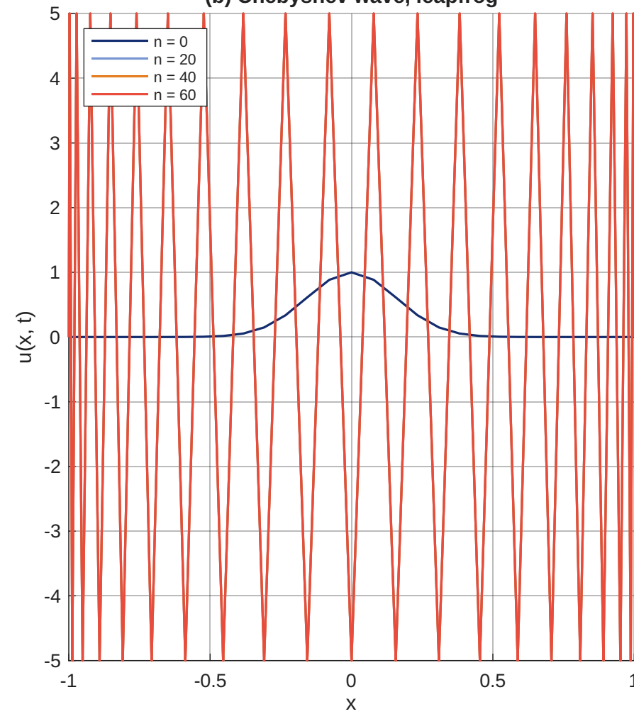
(b) Chebyshev wave, leapfrog
