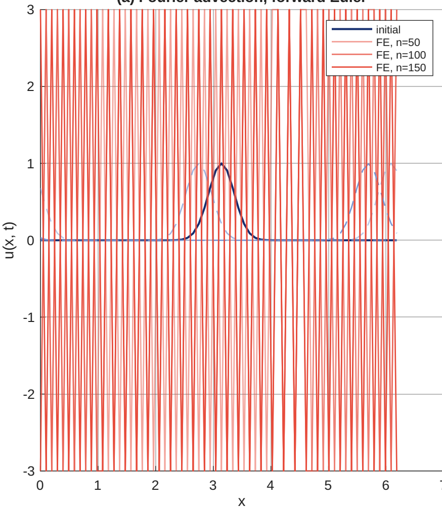
(a) Fourier advection, forward Euler
