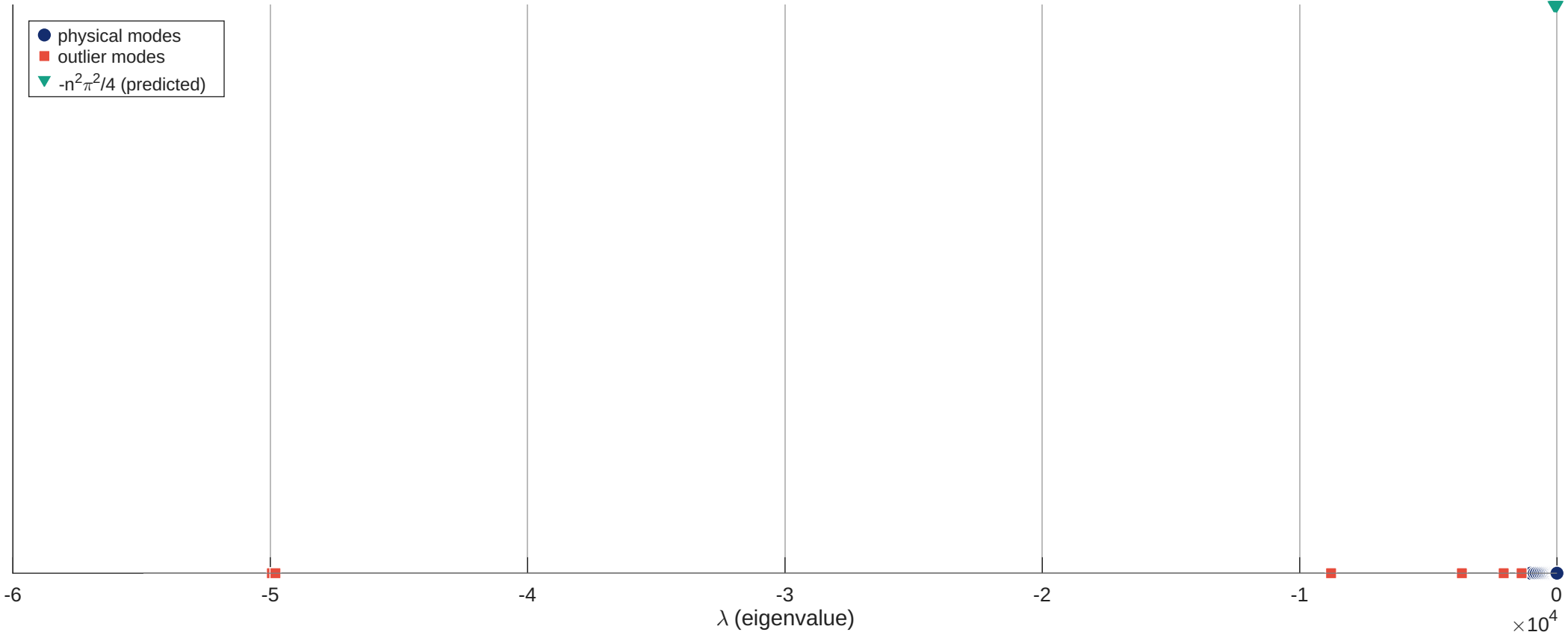
Eigenvalues of Chebyshev D^2 with Dirichlet BCs (N = 32)
