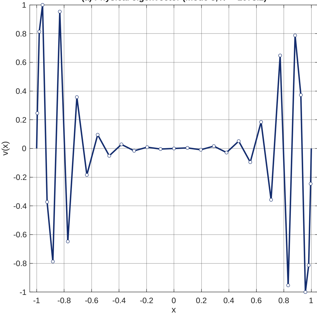
(a) Physical eigenvector (mode 8, \lambda = -2073.2 )
