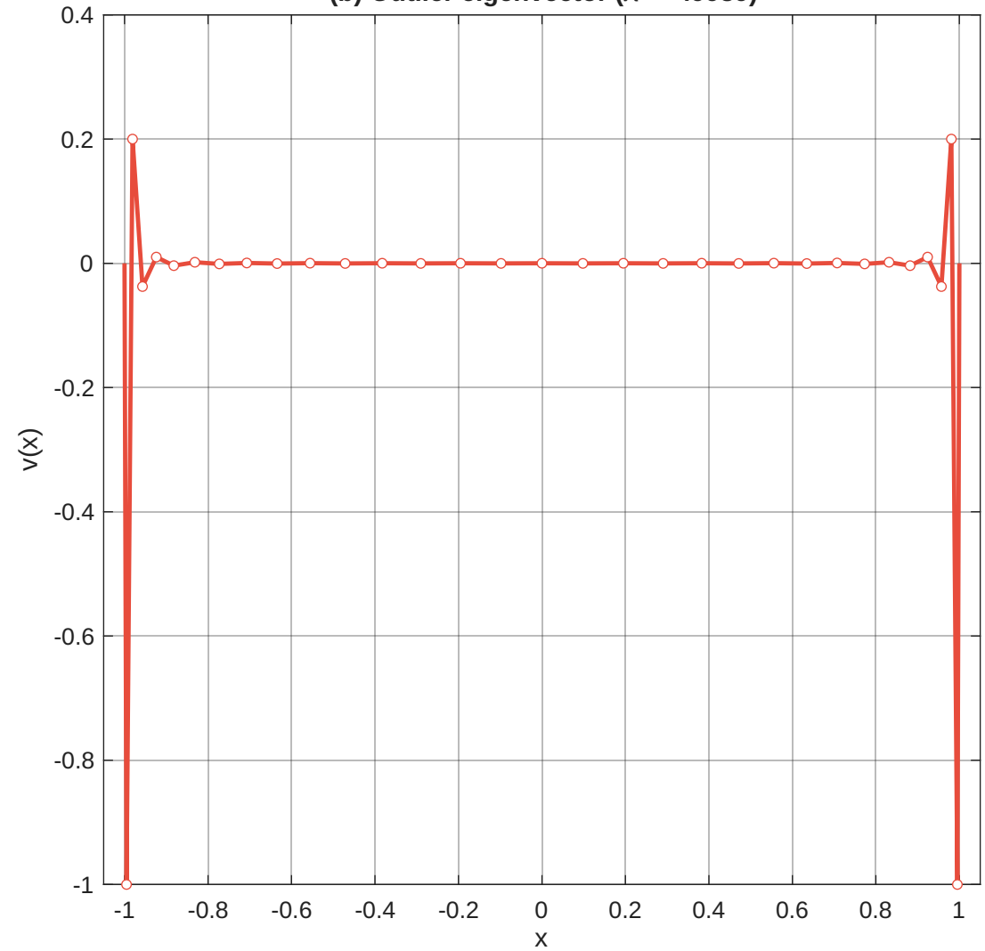
(b) Outlier eigenvector ( \lambda = -49939 )
