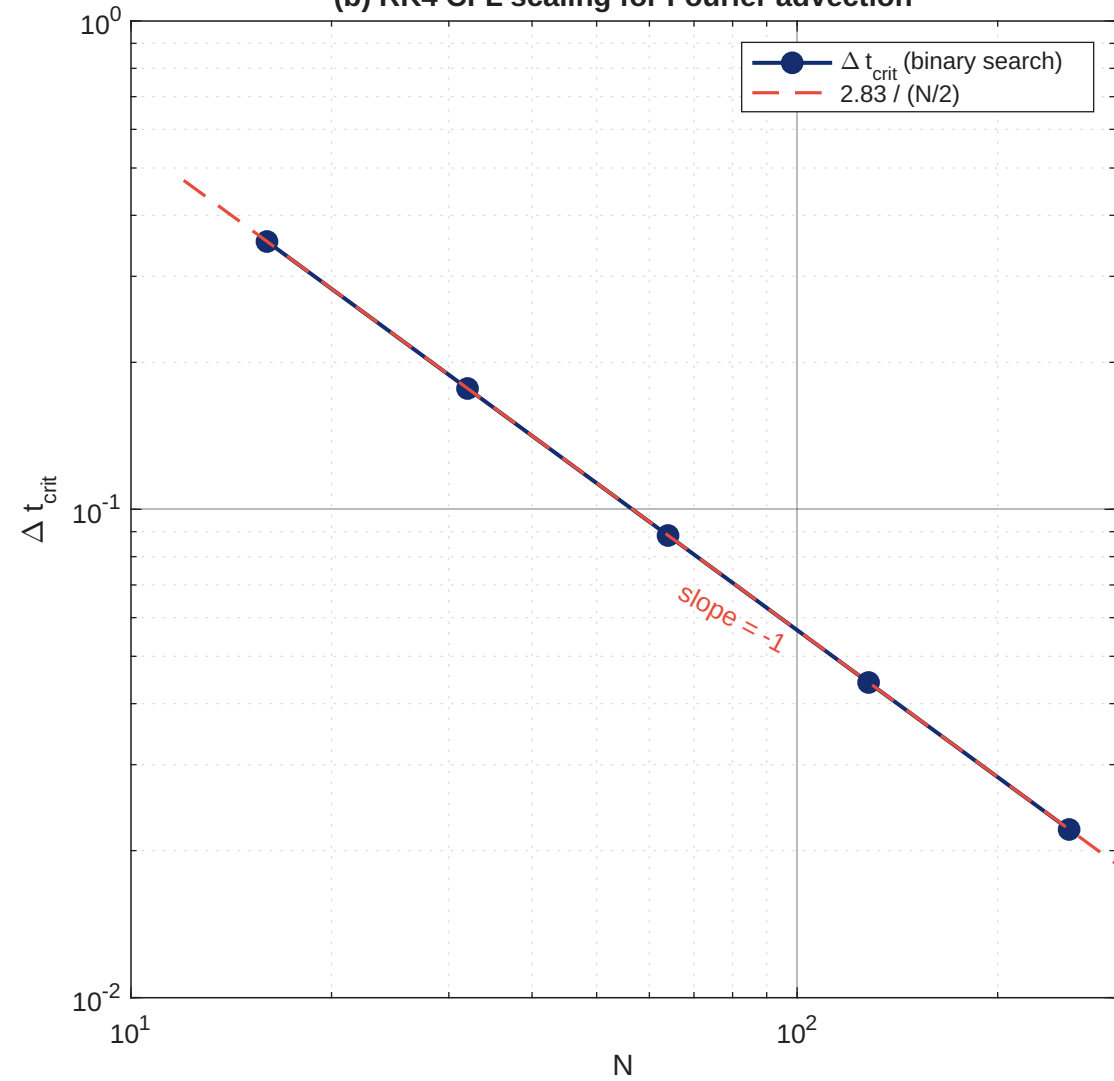
(b) RK4 CFL scaling for Fourier advection
