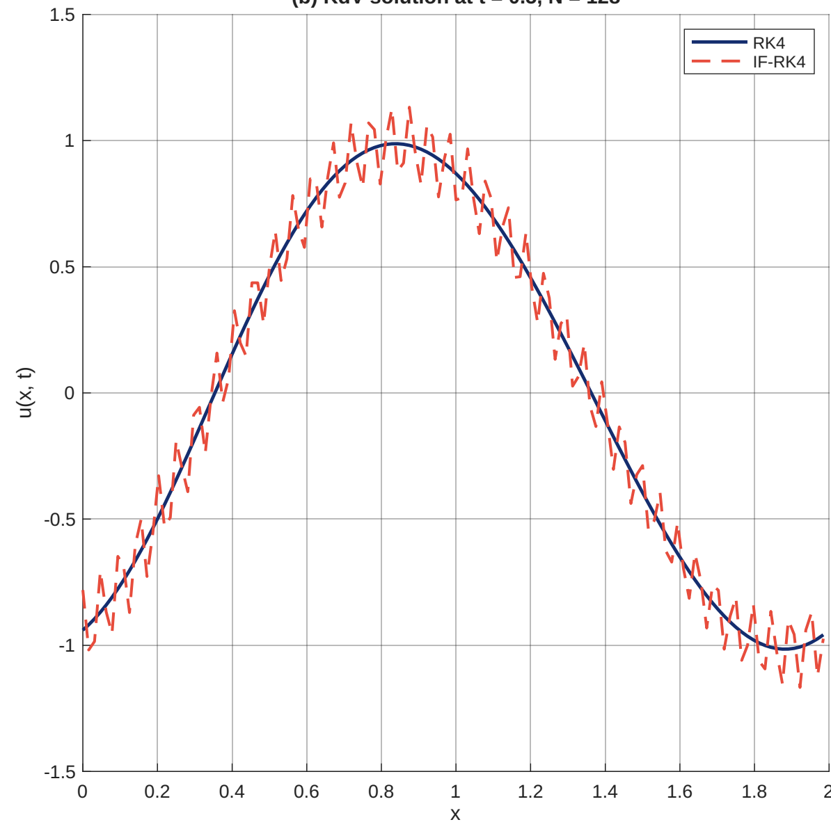
(b) KdV solution at t = 0.5 , N = 128
