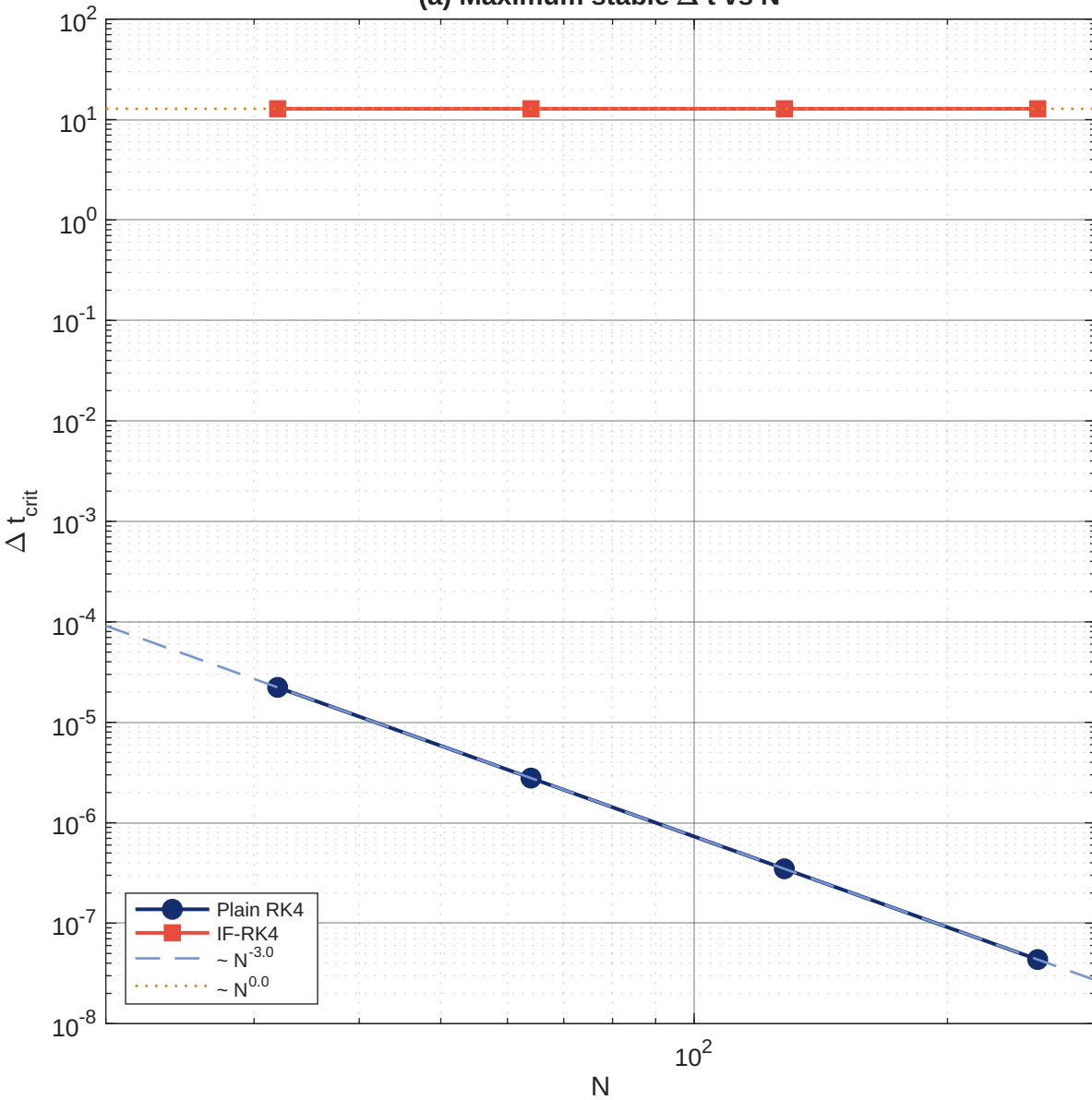
(a) Maximum stable \Delta t vs N
