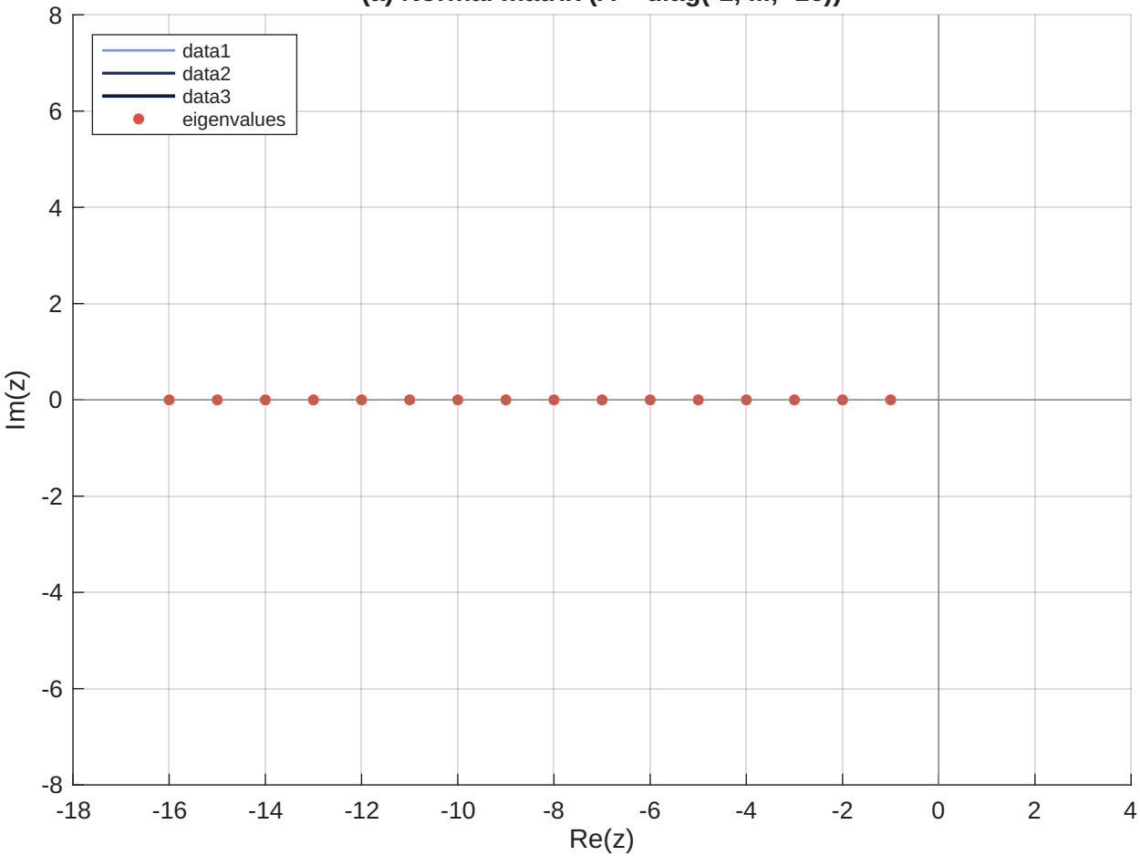
(a) Normal matrix ( A = \text{diag}(-1, \dots, -16) )
