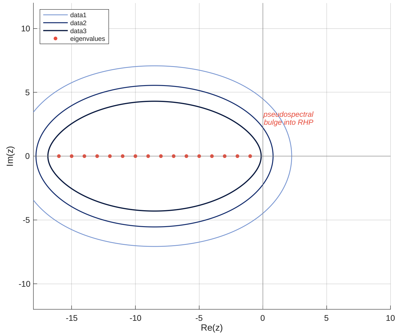
(b) Nonnormal ( A_{i,i+1} = 10 , same diagonal)
