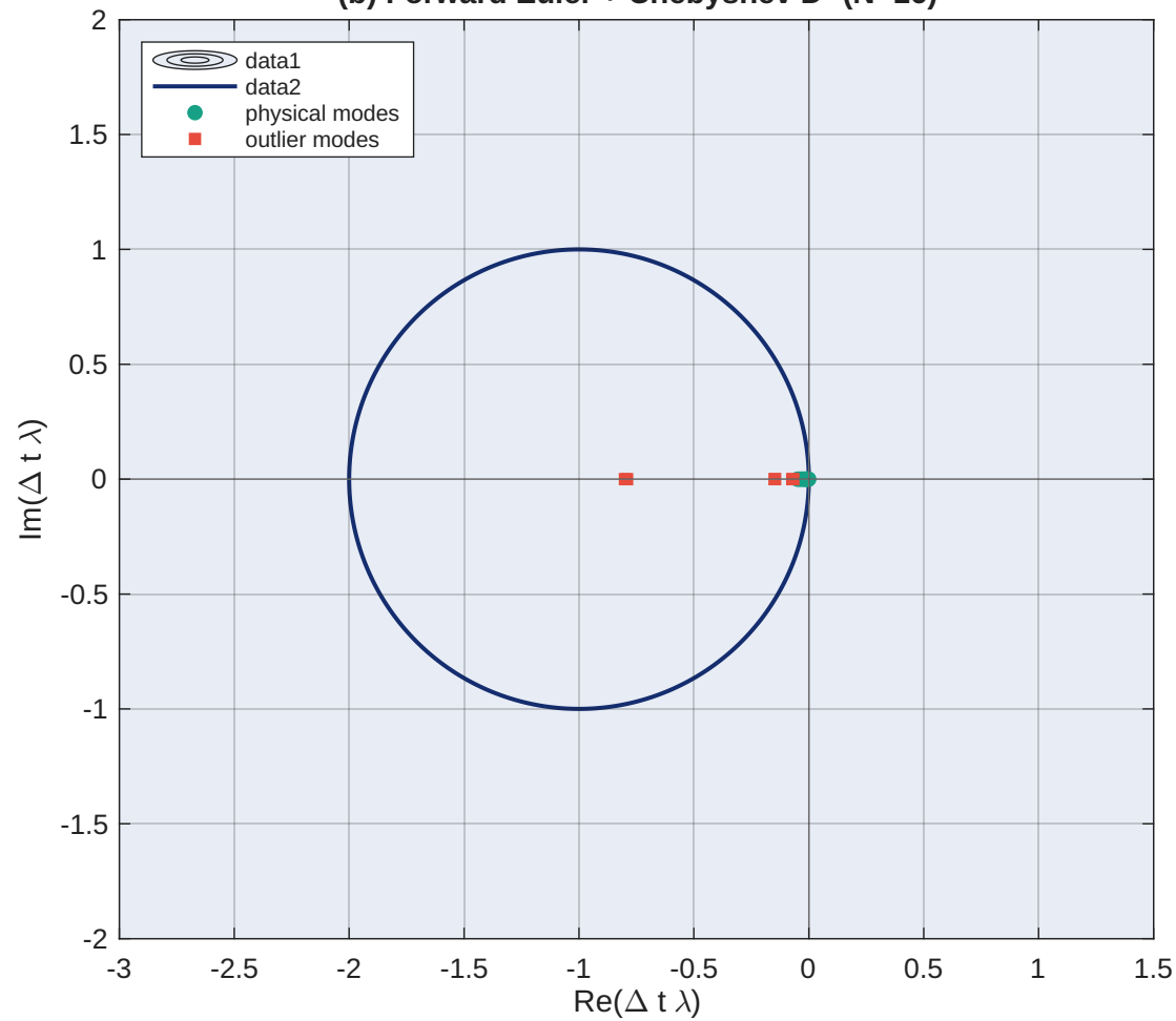
(b) Forward Euler + Chebyshev D^2 (N=16)
