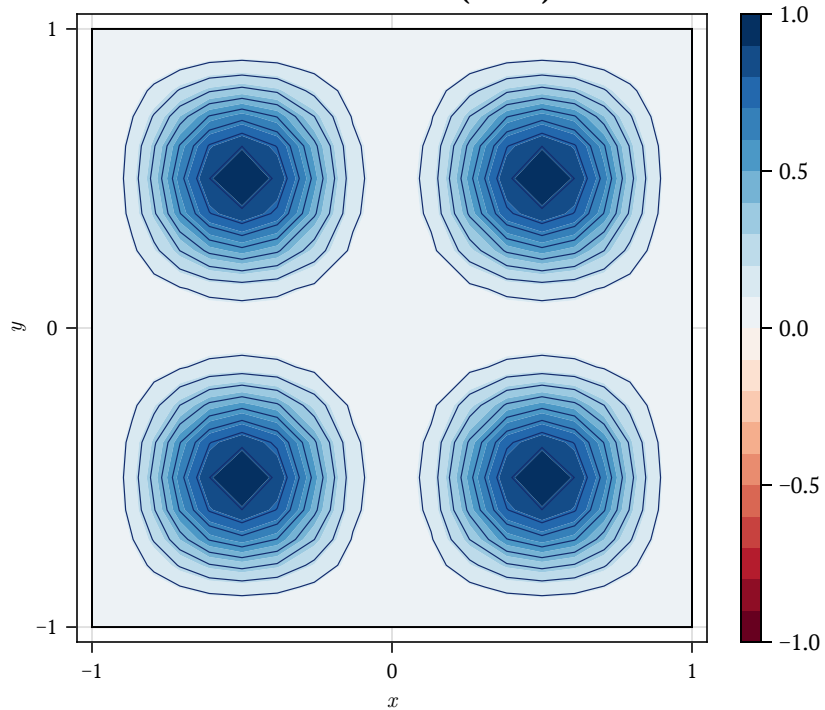
Numerical solution ( N = 24 )
