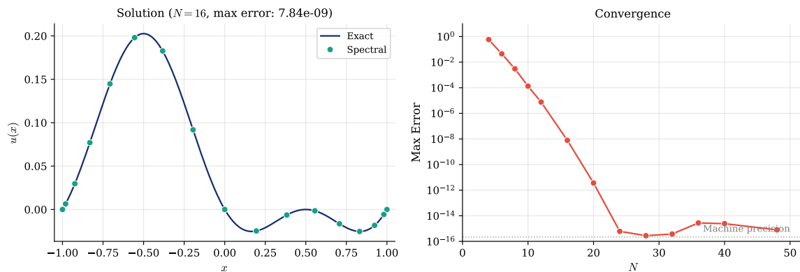
Figure 40: Solution of the 1D Poisson equation Equation 69. Left: numerical solution (circles) compared with exact solution (line) for N = 16 . Right: exponential convergence of the maximum error, reaching machine precision by N = 24 .
