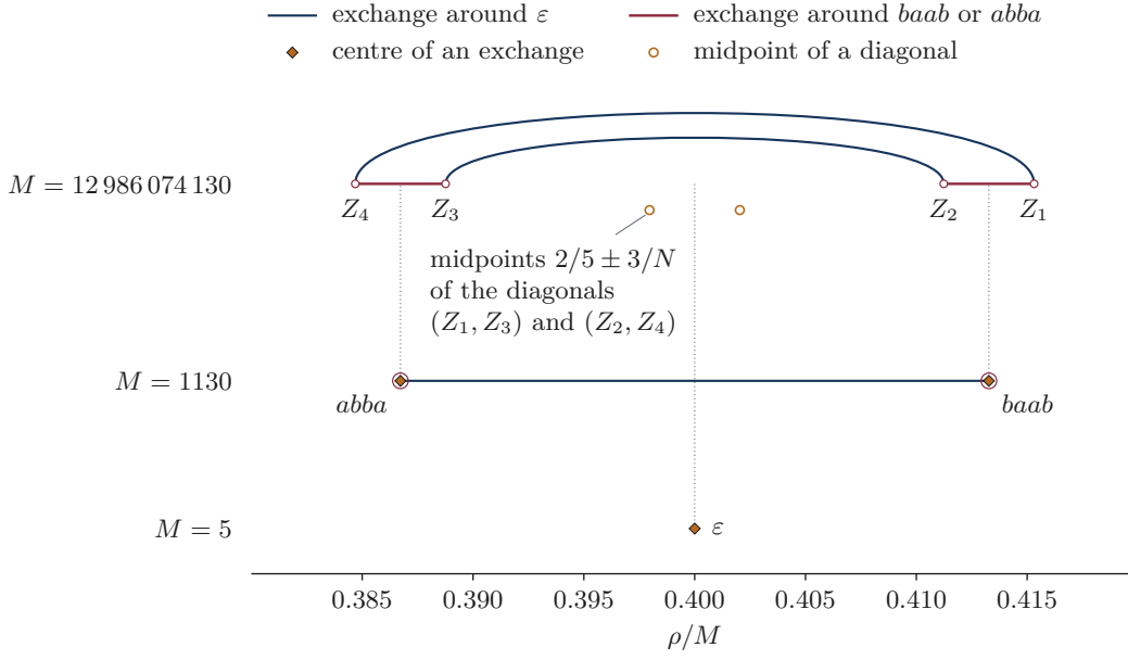
FIGURE 2. The square of corollary 4.15 for p = \varepsilon and W = V = (ba, ab) , in the plane of the ratio \rho/M and the label, at the labels 5, 1130 and 12 986 074 130. The two lower levels are drawn to scale. At the top level Z_1 and Z_2 lie at 467/1130 \pm 3/N and Z_3 and Z_4 at 437/1130 \pm 3/N , where N = 9 \cdot 1130^2 + 1 = 11\,492\,101 ; these offsets, about 2.6 \cdot 10^{-7} , are drawn enlarged, all by the same factor. The short rungs are the exchanges around baab and abba , each centred above its centre; the arcs are the exchanges around the empty word, centred at 2/5 like the rung below them. The diagonals (Z_1, Z_3) and (Z_2, Z_4) are not exchanges: their midpoints 2/5 \pm 3/N are the inner centre shifted by half the width of a short rung.
