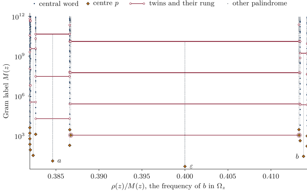
FIGURE 3. All palindromes with Gram label at most 10^{12} , placed by the ratio \rho/M and their Gram label M . The ratio \rho/M = t/(2t+1) increases with the slope t of lemma 6.2, and it is the frequency of the letter b in \Omega_z . Each horizontal segment joins two twins exchanged around a palindrome p (diamond), at the height of their common label; the dotted post shows that the segment is centred at the ratio \rho_p/M_p of p , which by lemma 6.2 is the lowest point between its ends. Ladders rise above the empty word, above a and above b . The two ringed diamonds, abba and baab , are twins themselves and centres of the exchanges at 12 986 074 130, the square of figure 2. No central word lies on a rung.
