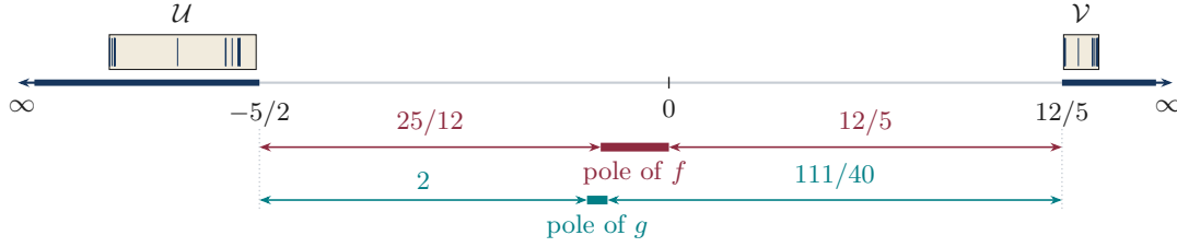
FIGURE 1. The cusp coordinate z at the empty directive, where f(z) = -3 - 1/z and g(z) = 5/2 - 1/(4z + 2) . Every column of a nonempty word lies on one of the two rays of \mathcal{H} (thick), and the terminal column is the point at infinity. The poles of f and g lie in the gap between the rays; the bars below the axis show the intervals [-5/12, 0] and [-1/2, -3/8] that contain them for every directive, and the arrows show the four distances of table 1, measured from the ends of these ranges. The shaded boxes are the cylinders \mathcal{U} and \mathcal{V} of (29), and the ticks above the axis are the columns of all words of length at most nine.
