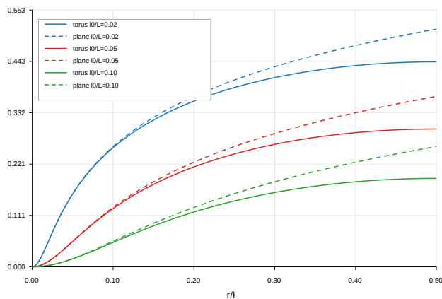
FIG. 1: Axial finite-volume T-duality potential (78) on the square torus. The solid curves show the zero-mode-subtracted toroidal pair energy \mathcal{U}_{\text{ax}}(\xi; \mathfrak{a}) = \Delta V_{L, \ell_0}(r, 0)/Q^2 as a function of \xi = r/L , for \mathfrak{a} = \ell_0/L \in \{0.02, 0.05, 0.10\} . The dashed curves show the corrected infinite-plane reference potential (79). At small separations, the toroidal result approaches the infinite-plane potential, while at separations of order L , the finite geometry and zero-mode subtraction produce a bounded periodic interaction.
