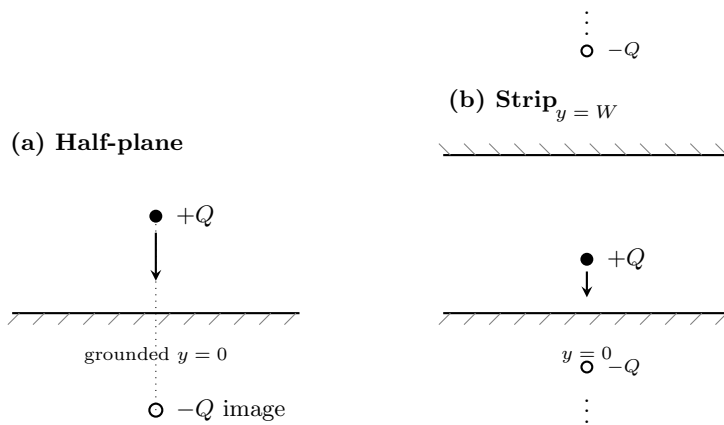
FIG. 2: Image construction behind Proposition IV.2. In the half-plane a single mirror charge enforces the grounded boundary. In the strip the Dirichlet kernel is generated by an infinite alternating tower of images at \pm y + 2pW . The arrows indicate the direction of the boundary self-force described in Corollary IV.1. The zero-point length \ell_0 smooths the force near the grounded walls.
