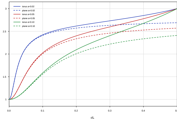
FIG. 3: Potential-based running interaction dimension for the corrected infinite plane and for the square torus. The horizontal axis is \xi = r/L , and \mathbf{a} = \ell_0/L . Solid curves show the toroidal result \mathbb{D}_{\Delta, T^2}(\xi; \mathbf{a}, \hat{x}) obtained from the zero-mode-subtracted axial mode sum (see Eq. (131)), while dashed curves show the corrected infinite-plane reference \mathbb{D}_{\Delta}^{(\infty)}(\xi/\mathbf{a}) . All curves approach the ultraviolet limit \mathbb{D}_{\Delta} \rightarrow 1 as \xi \rightarrow 0 . The finite-torus curves saturate to \mathbb{D}_{\Delta} = 3 at the maximally separated axial point \xi = 1/2 , where the potential is smooth and periodic, whereas the infinite-plane reference approaches 3 only through the logarithmic large-distance limit.
