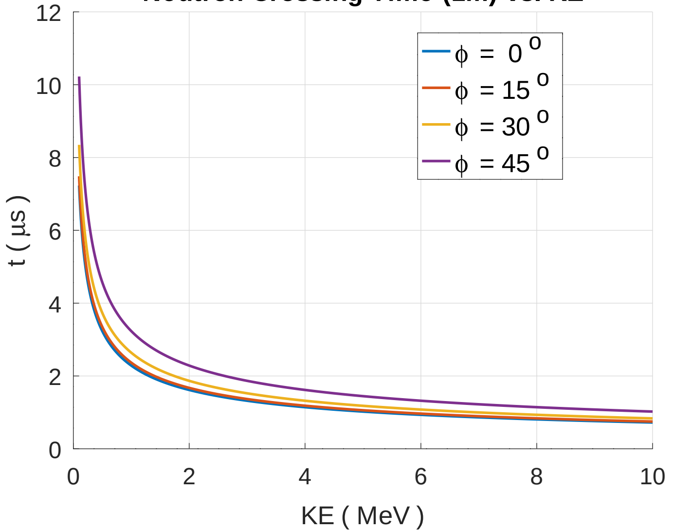
Neutron Crossing Time (1m) vs. KE
