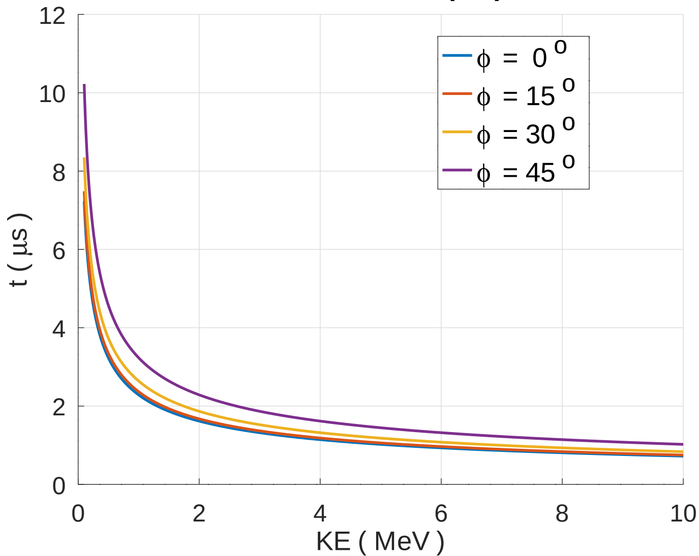
Neutron Travel Time (1m) vs. KE
