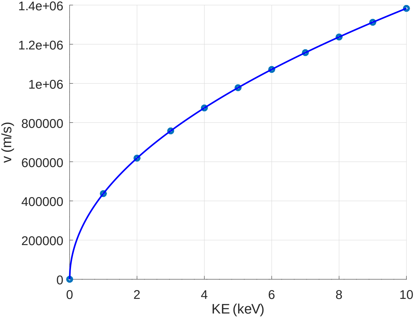
Neutron Speed vs. KE
