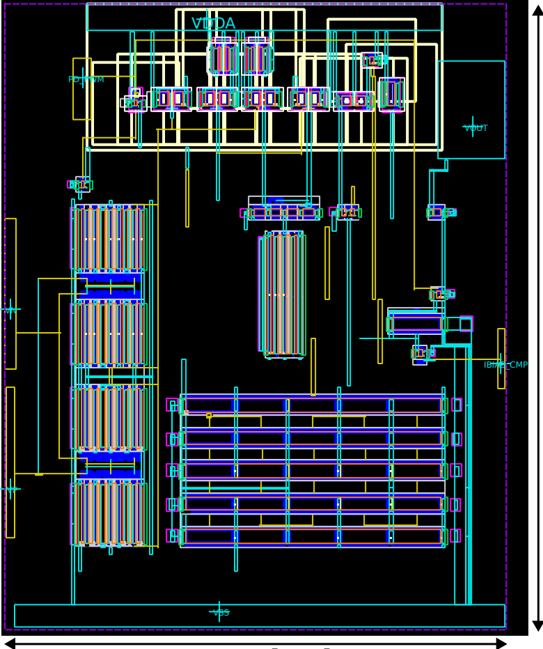
(a) Baseline layout of the comparator
