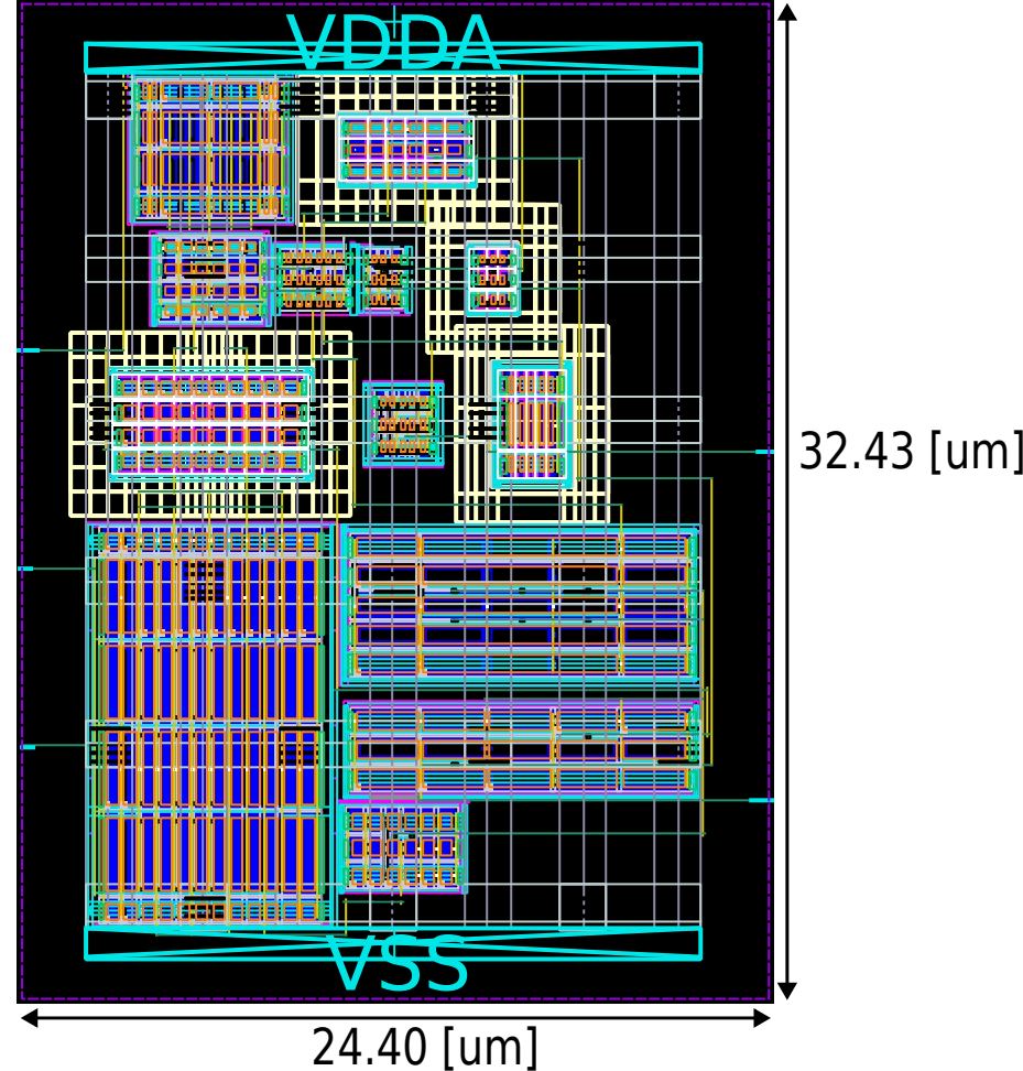
(b) Proposed layout of the comparator
