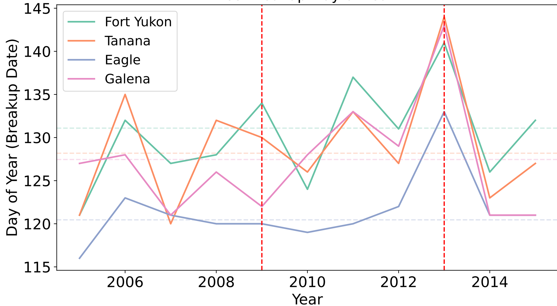
Ice Breakup Day of Year
