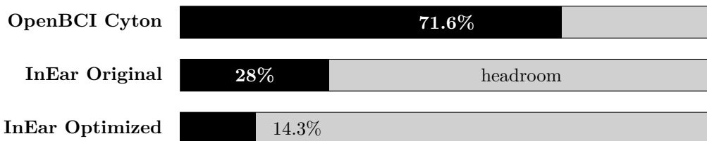
Figure 6: Bandwidth utilization comparison (bar chart). Each bar represents the percentage of the serial link capacity used.
