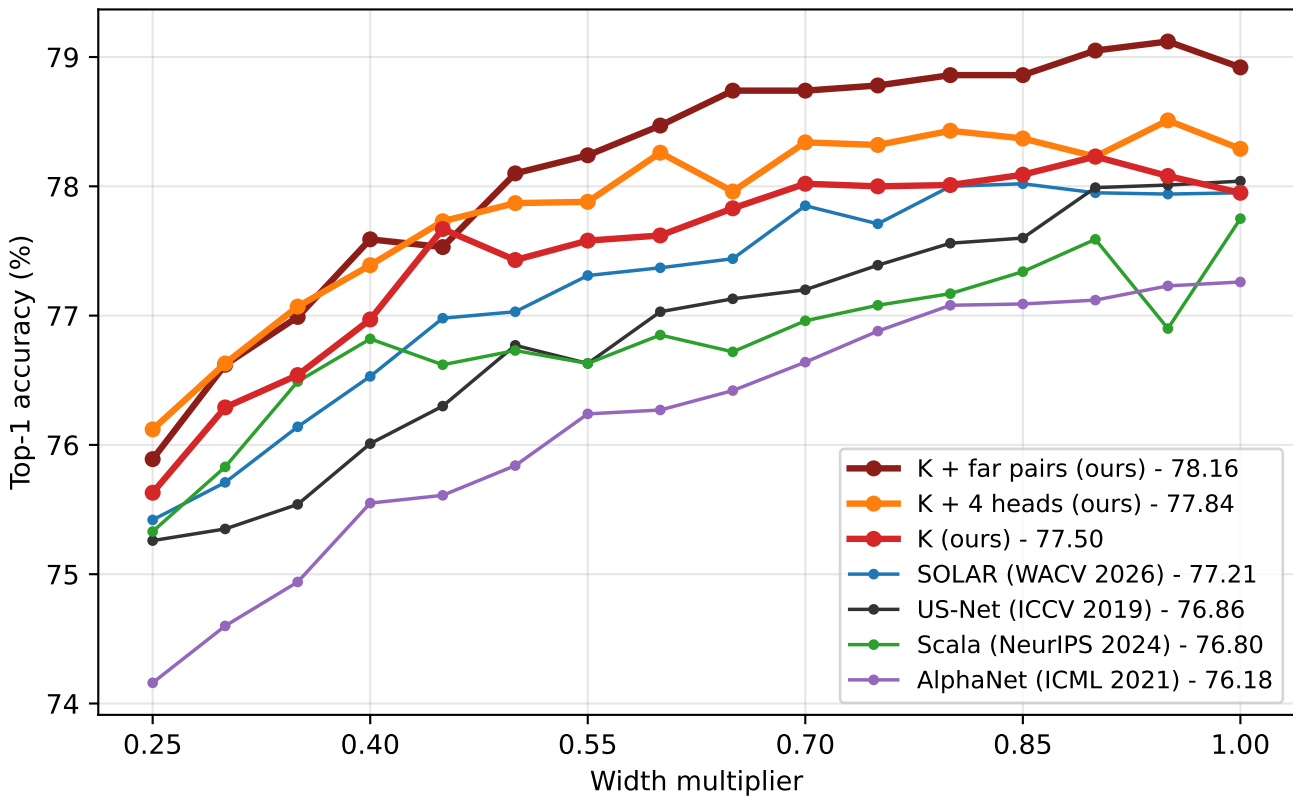
ResNet-50, CIFAR-100: accuracy against width (legend: mean over 16 widths)
