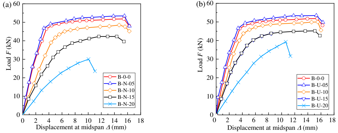
Fig. 17 Load-mid-span deflection relationship of specimens subject to four-point bending test, (a) non-uniform corrosion, and (b) uniform corrosion.
