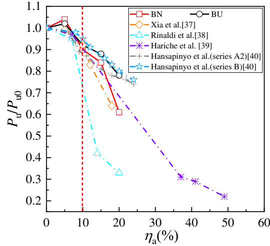
Fig. 19 Degradation model of flexural capacity versus the corrosion degree of tensile reinforcement for RC beams.
