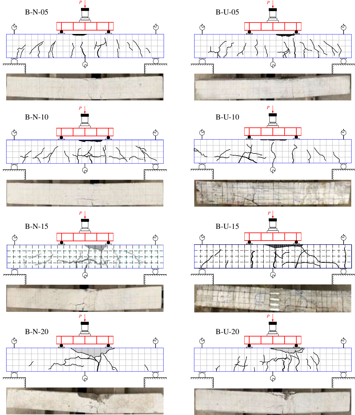
Fig. 13 Load-induced cracks and failure modes of RC beams.
