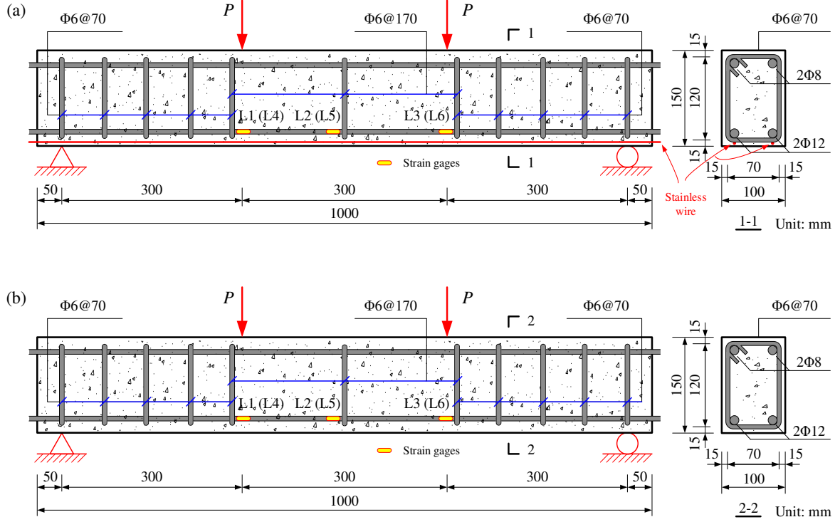
Fig. 1 Dimensions of the specimens subjected to (a) modified accelerated corrosion with auxiliary electrode, and (b) traditional accelerated corrosion.
