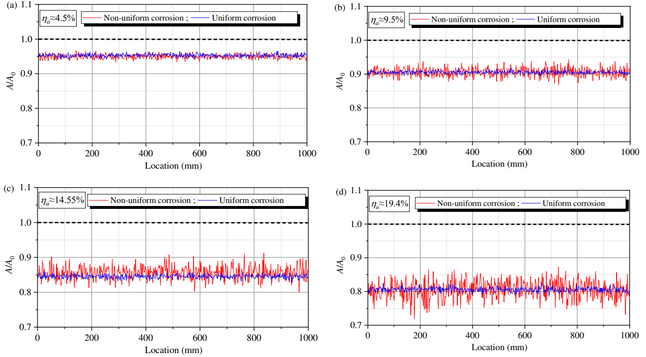
Fig. 8 Distribution of residual cross-sectional area of longitudinal reinforcements relative to its original in RC beams subjected to non-uniform and uniform accelerated corrosion methods.
