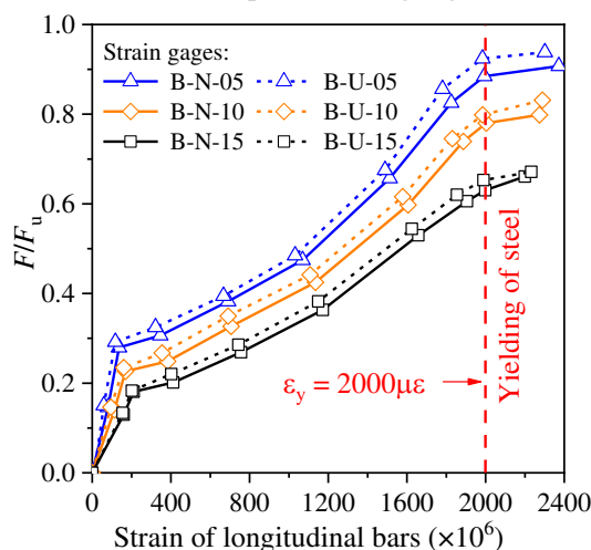
Fig. 14 The relationships between the load and the strain of longitudinal tensile reinforcements.
