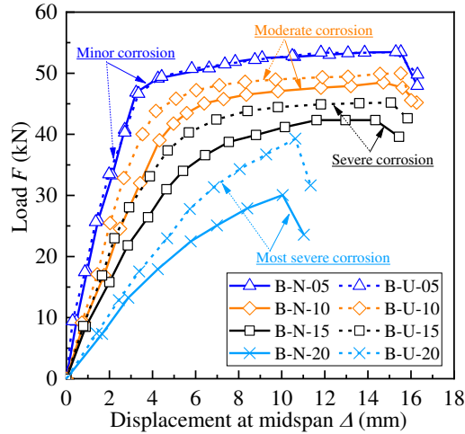
Fig. 18 Comparison of load-mid-span displacement curves for two different accelerated corrosion methods
