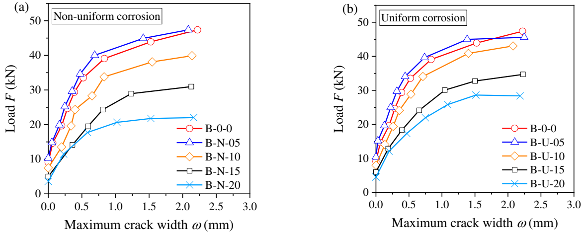
Fig. 11 Load-maximum crack width relationship of specimens subject to four-point bending test, (a) non-uniform corrosion, and (b) uniform corrosion.
