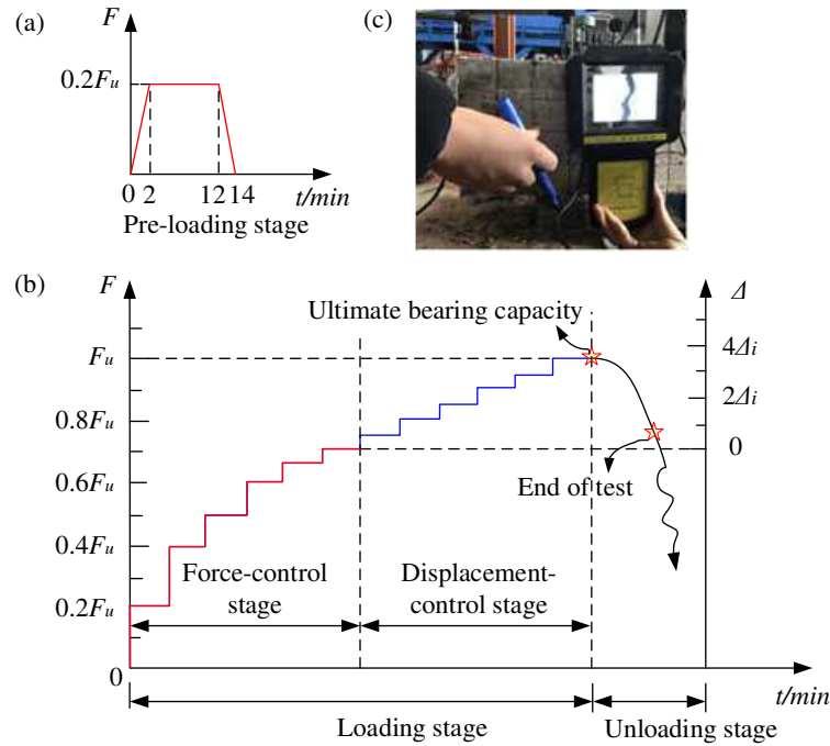
Fig. 5 Loading process, where F_u is the ultimate bearing capacity and \Delta_i is the displacement increment at displacement-control stage.
