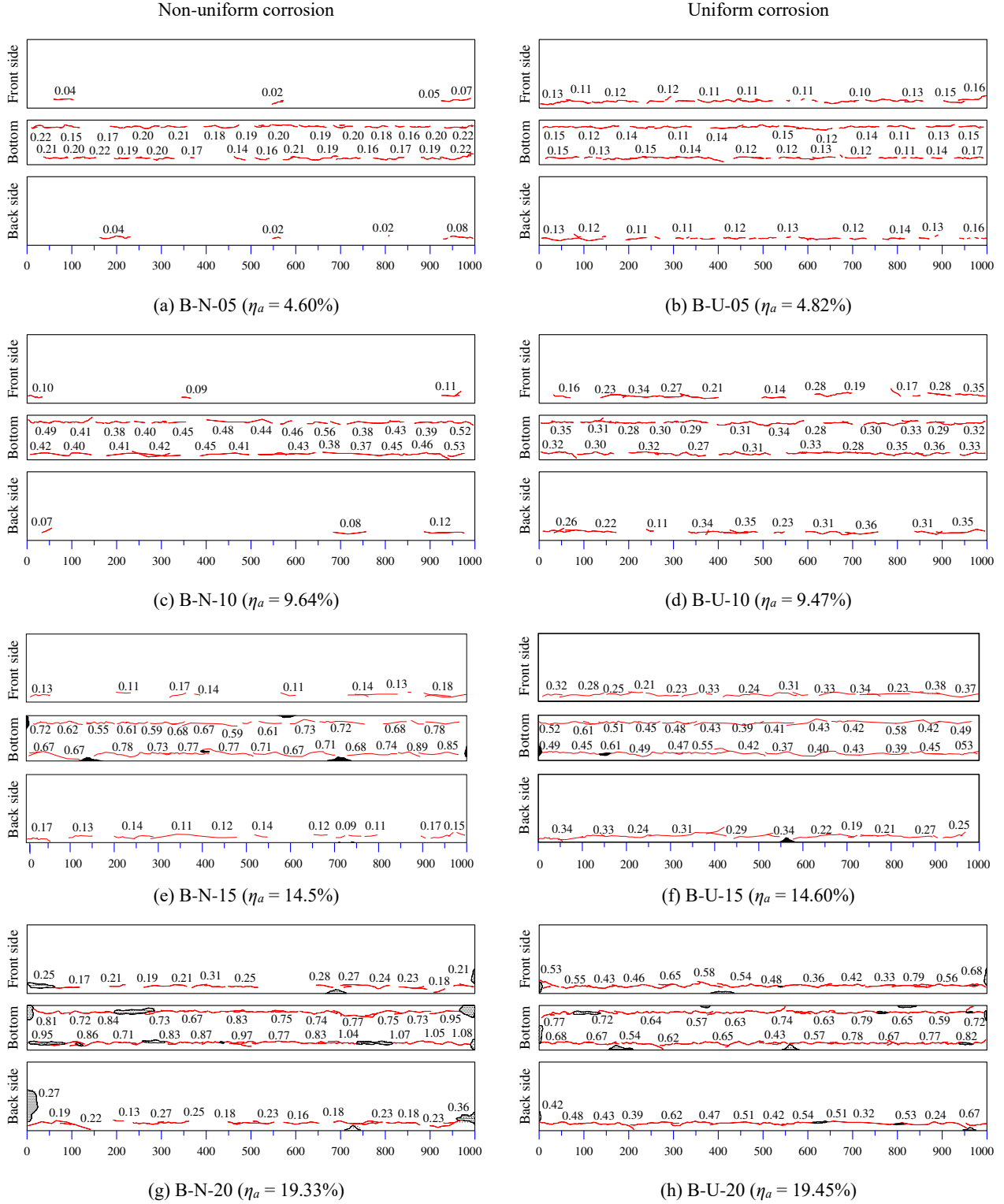
Fig. 10 Cracking maps of corroded RC beams subjected to different accelerated corrosion methods.
