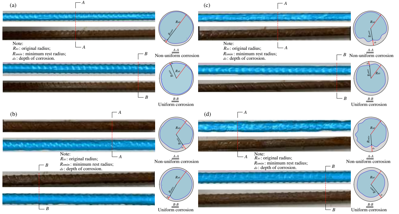
Fig. 7 Corrosion morphology around the circumference of longitudinal reinforcements in the cases of (a) \eta_a = 4.6\% , (b) \eta_a = 9.5\% , (c) \eta_a = 14.5\% , (d) \eta_a = 19.4\% subjected to non-uniform and uniform accelerated corrosion methods.
