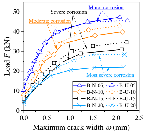
Fig. 12 Comparison of load-maximum crack width curves for two different accelerated corrosion methods
