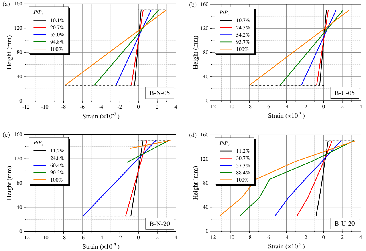
Fig. 16 Strain distribution of concrete along the height in the cases of different reinforcement corrosion levels. (a) and (b): \eta_d = 5\% ; (c) and (d): \eta_d = 20\% .
