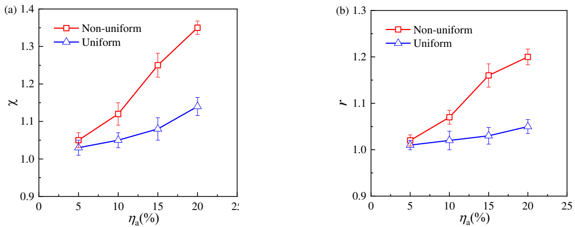
Fig. 9 The values of (a) the non-uniformity of longitudinal reinforcements circumferentially ( \chi ) and (b) the non-uniformity of longitudinal reinforcements longitudinally ( r ) with increasing corrosion degree.
