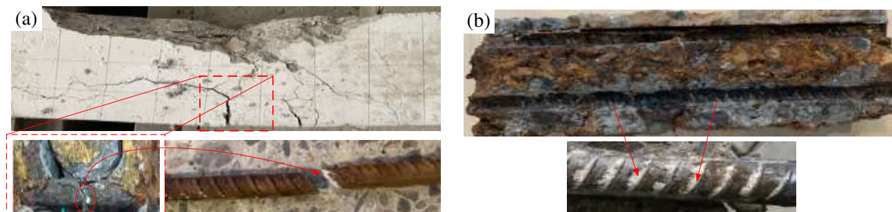
Fig. 15 Details demonstrating the failure of specimens (a) B-N-20 and (b) B-U-20
