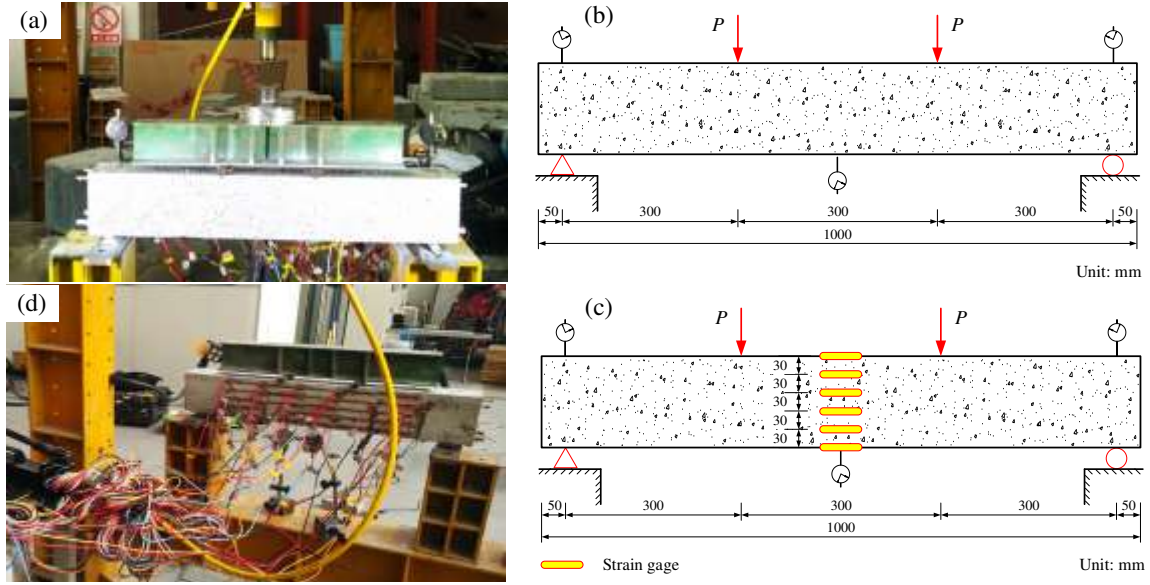
Fig. 6 Setup for the four-point bending test.
