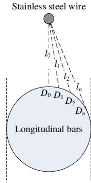
Fig. 2 Illustration for the position of longitudinal reinforcements and stainless steel wire in the accelerated non-uniform corrosion method
