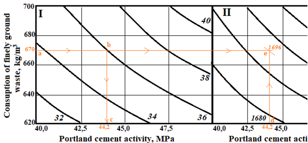
Fig. 4. Nomogram for selecting the composition and predicting the properties of fiber-reinforced concrete at the optimal consumption of PVC fiber equal to 5.90...6.0 kg/m3.
