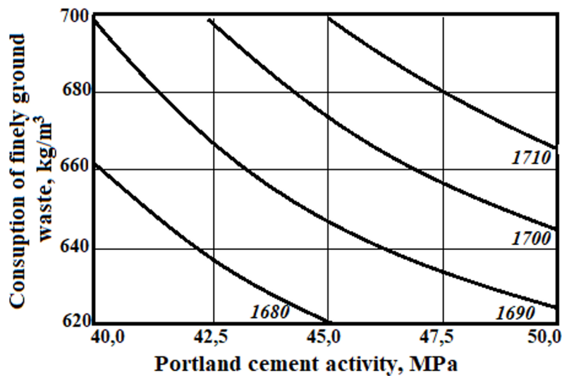
Fig. 3. Dependence of the average density of fiber-reinforced concrete samples on the activity of Portland cement and the consumption of finely ground waste at the optimal consumption of PVC fiber equal to 5.90...6.0 kg/m³.
