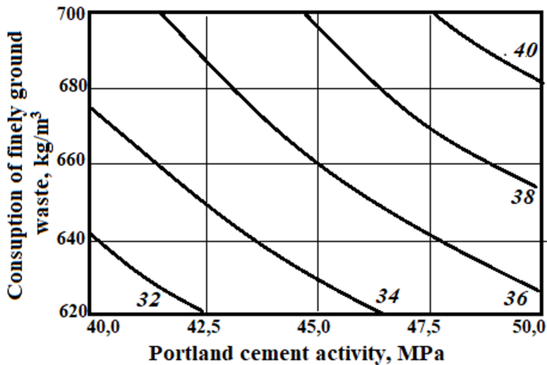
Fig. 2. Dependence of the compressive strength of fiber-reinforced concrete samples on the activity of Portland cement and the consumption of finely ground waste at the optimal consumption of polyvinyl chloride fiber equal to 5.90...6.0 kg/m 3 .
