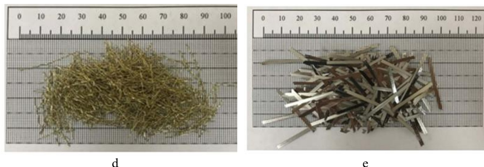
Fig. 1. Reinforcing fibers: a – polypropylene fiber; b – basalt fiber; c – glass fiber; g – stone wool fiber; d – steel fiber; e – composite fiber
