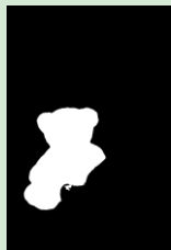
Reflection Mask
