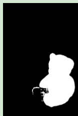
Object Mask
