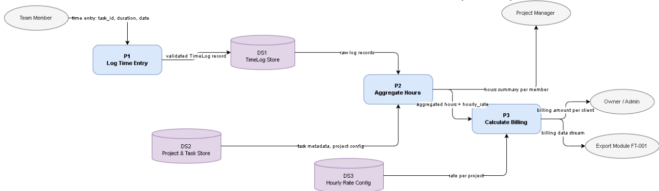
DATA FLOW DIAGRAM — TIME TRACKING (FT-002)
