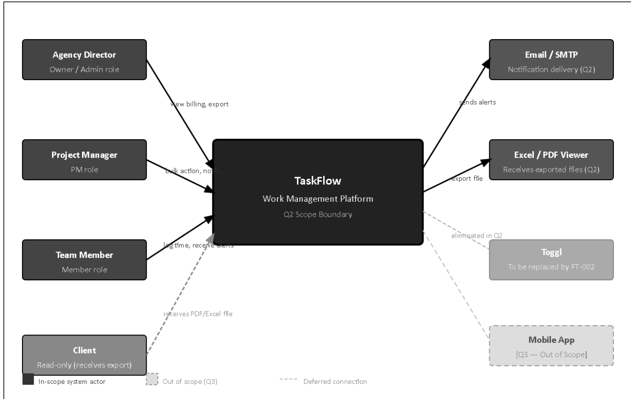
Diagram 1: System Context — TaskFlow Q2 Boundary (Level 0)
