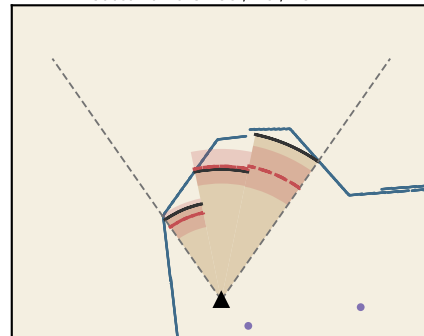
nearest wall 893 mm sector errors 286 / 26 / 79 mm
