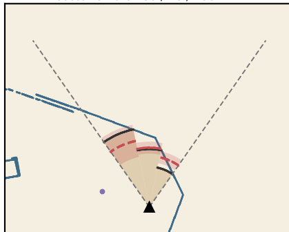
nearest wall 522 mm sector errors 135 / 18 / 150 mm
