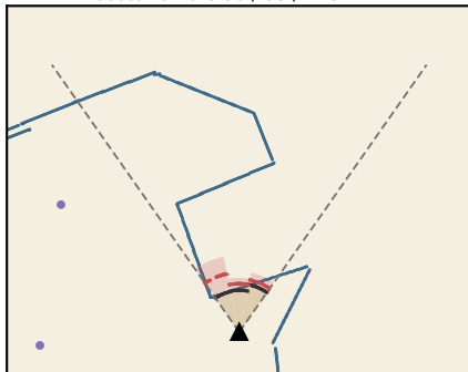
nearest wall 330 mm sector errors 38 / 53 / 145 mm
