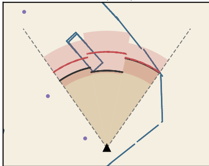
nearest wall 1381 mm sector errors 9 / 335 / 187 mm
