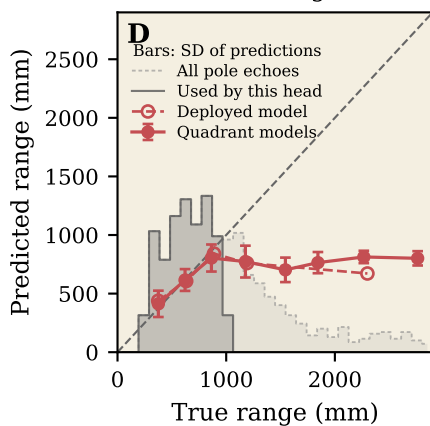
Pole range
