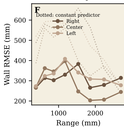
Wall depth
