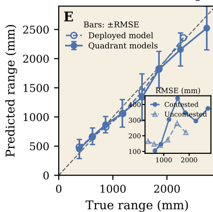
Nearest-reflector range
