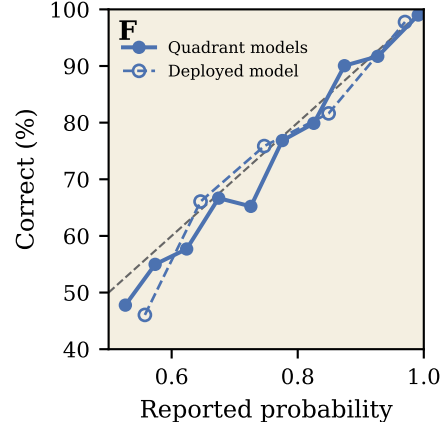
Reliability (ECE 0.020)
