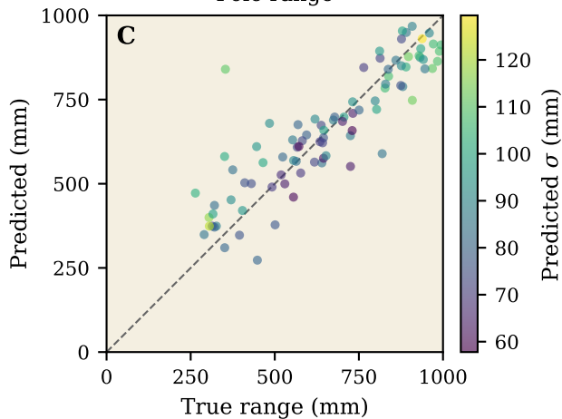
Pole range
