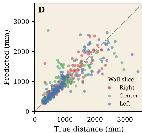
Wall depth
