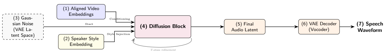
Σχήμα 2: The Generation by Diffusion part of the proposed method
