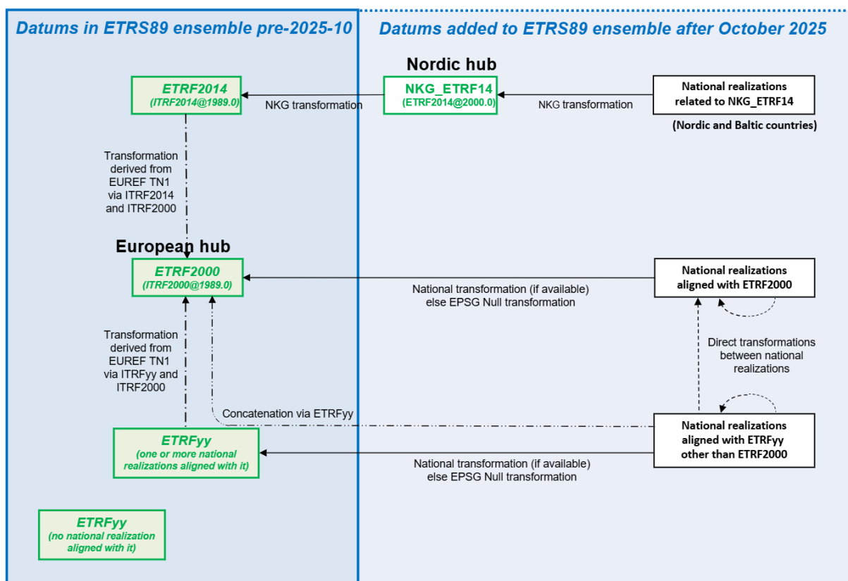
Figure 1: Relationships between realizations of ETRS89 in the EPSG Dataset.
