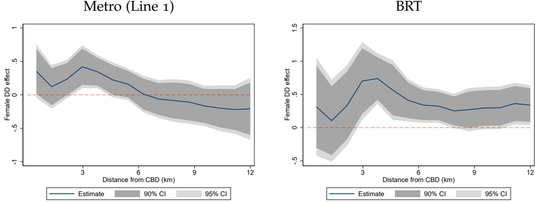
Figure 11: Rolling-window DD on female labor income relative to male.
