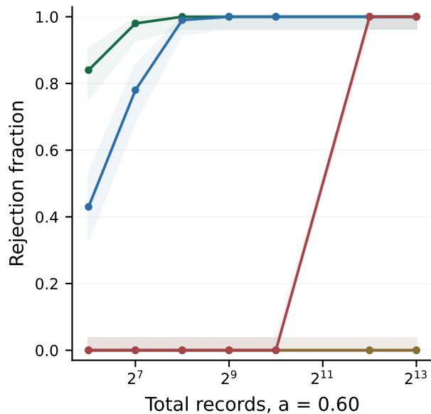
b Sample cost of valid exclusion
