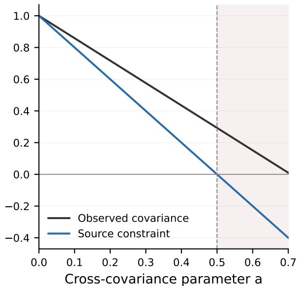
a Calibration exposes a boundary
