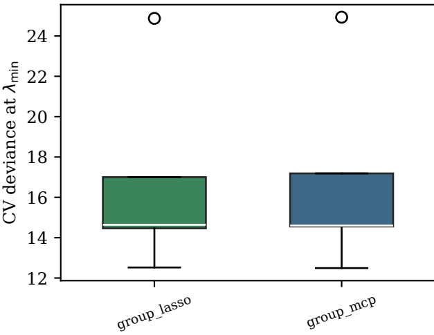
F6 — Real-dataset CV deviance, per fold bardet (n=189, p=16, family=gaussian) pbc (n=276, p=17, family=cox)
