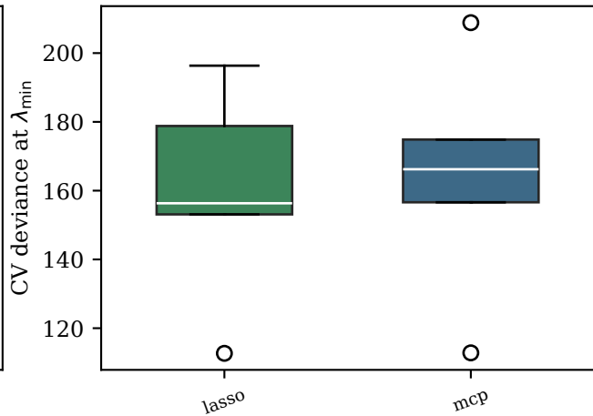
F6 — Real-dataset CV deviance, per fold bardet (n=189, p=16, family=gaussian) pbc (n=276, p=17, family=cox)
