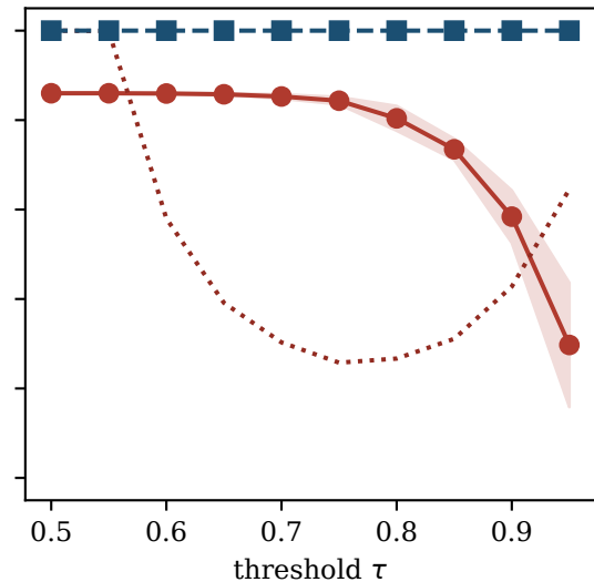
F8 — Stability selection: FDR vs MB bound, and power
