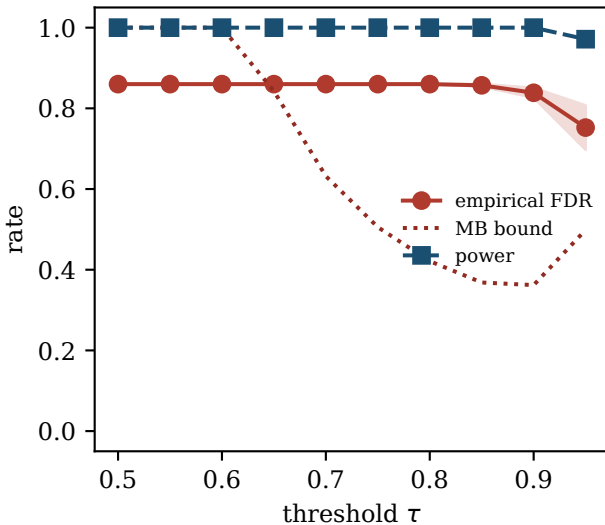
F8 — Stability selection: FDR vs MB bound, and power
