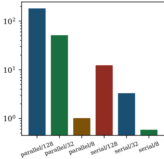
F9 — Screening + Jacobi-parallel ablation (criterion microbench)
