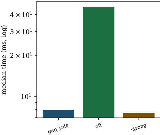
F9 — Screening + Jacobi-parallel ablation (criterion microbench)
