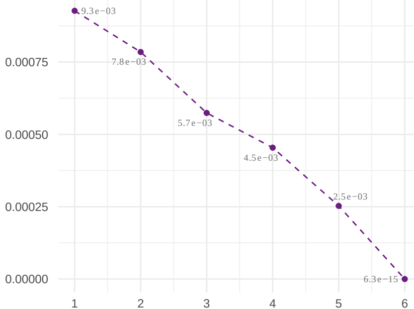
MAESD
