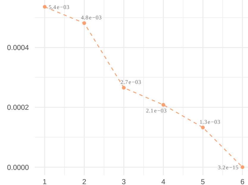
MAESD
