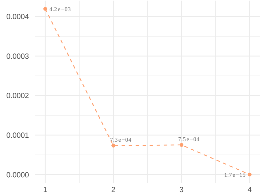
MAESD
