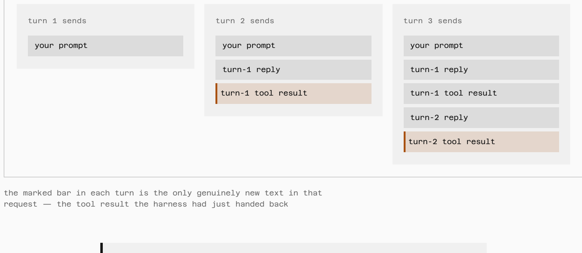
fig. 5 · what three consecutive turns actually send
