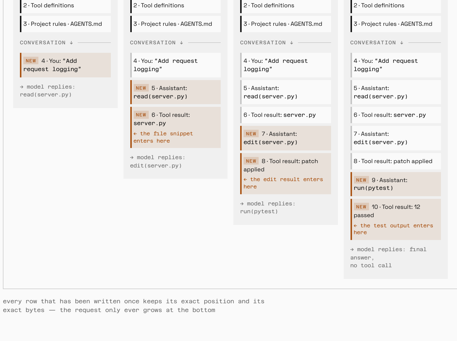
fig. 6 · four turns of one cycle, row by row
